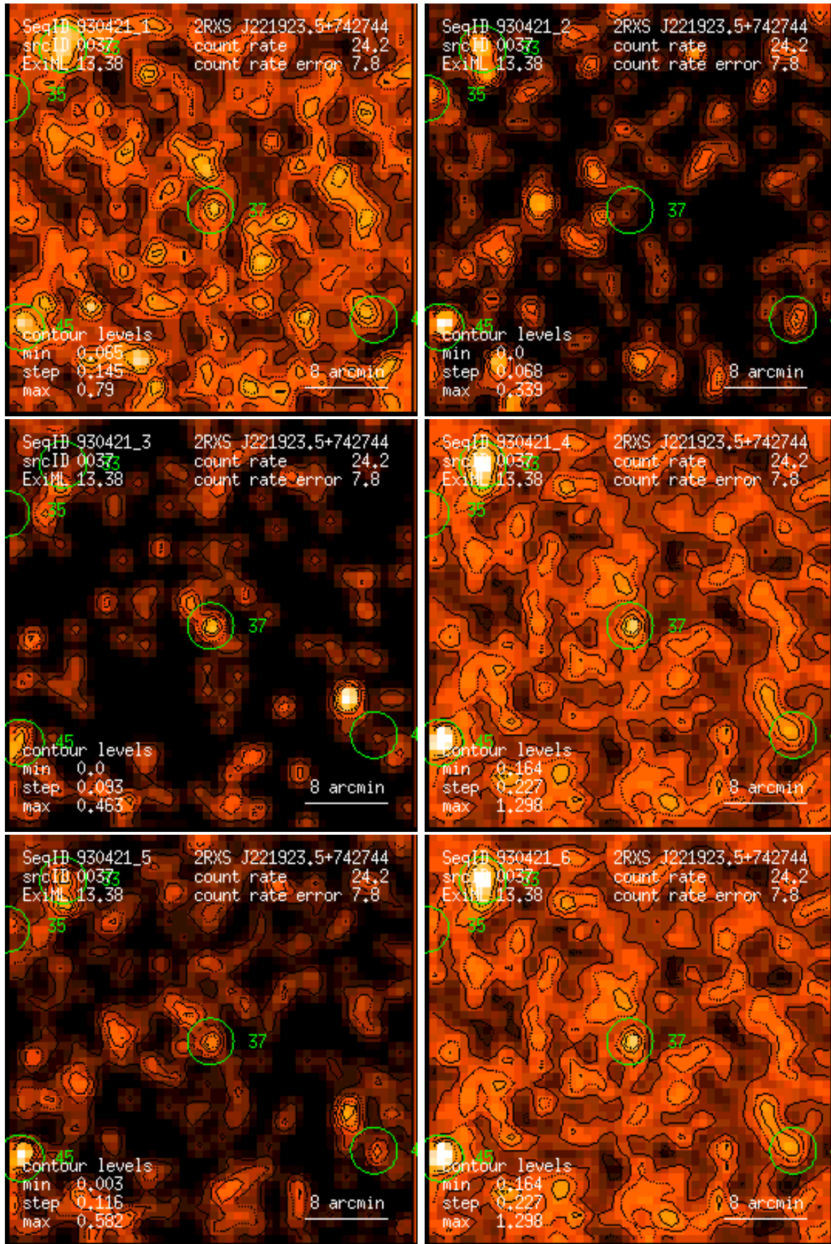
Figure 37: RASS 930421: detection 0037: band rate images, Gaussian filter: (1) PSPC channels 11 – 41, (2) 52 – 90, (3) 91 – 201, (4) 11 – 235, (5) 52 – 201, (6) 11 – 201. Broad band rates in counts/ks. Band rate contour levels in counts/ks/arcmin 2 .
