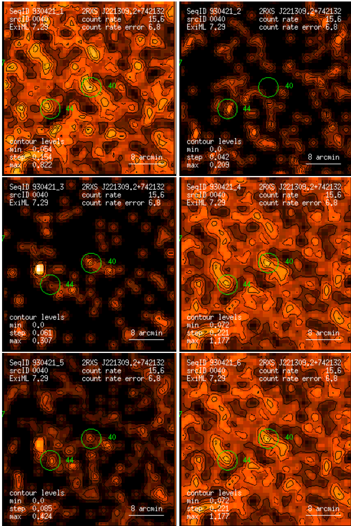
Figure 40: RASS 930421: detection 0040: band rate images, Gaussian filter: (1) PSPC channels 11 – 41, (2) 52 – 90, (3) 91 – 201, (4) 11 – 235, (5) 52 – 201, (6) 11 – 201. Broad band rates in counts/ks. Band rate contour levels in counts/ks/arcmin 2 .
