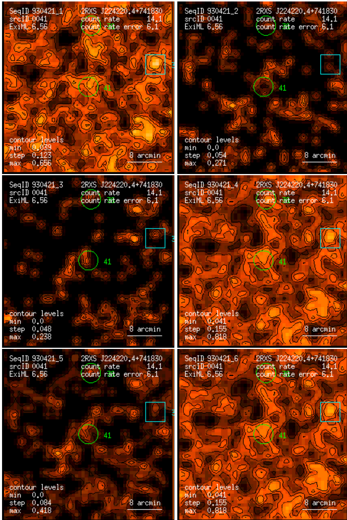
Figure 41: RASS 930421: detection 0041: band rate images, Gaussian filter: (1) PSPC channels 11 – 41, (2) 52 – 90, (3) 91 – 201, (4) 11 – 235, (5) 52 – 201, (6) 11 – 201. Broad band rates in counts/ks. Band rate contour levels in counts/ks/arcmin 2 .
