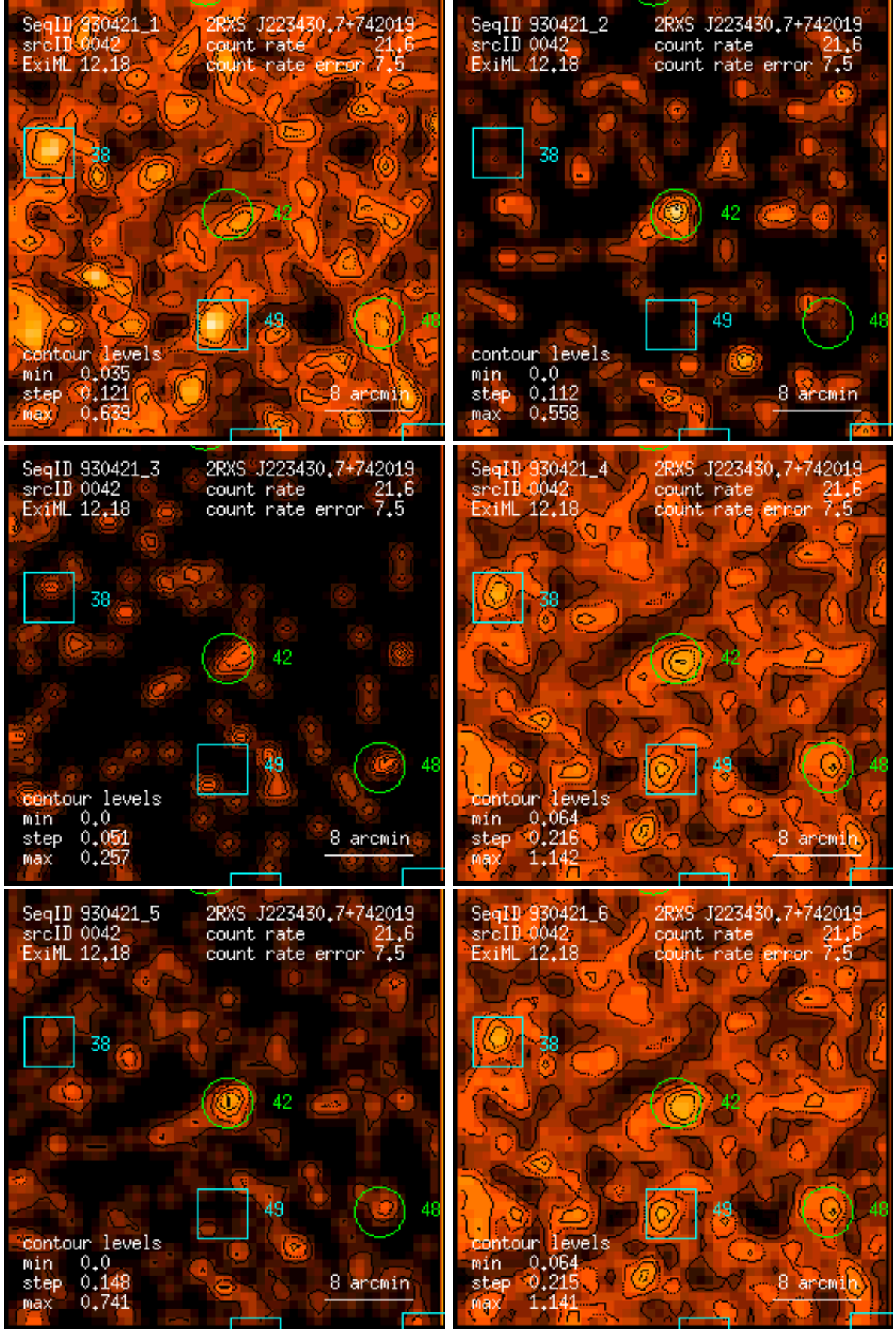
Figure 42: RASS 930421: detection 0042: band rate images, Gaussian filter: (1) PSPC channels 11 – 41, (2) 52 – 90, (3) 91 – 201, (4) 11 – 235, (5) 52 – 201, (6) 11 – 201. Broad band rates in counts/ks. Band rate contour levels in counts/ks/arcmin 2 .
