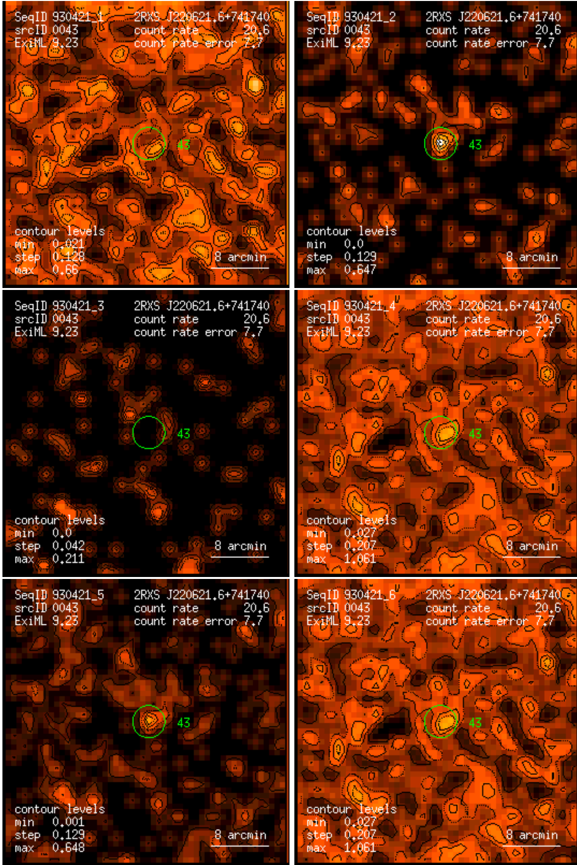
Figure 43: RASS 930421: detection 0043: band rate images, Gaussian filter: (1) PSPC channels 11 – 41, (2) 52 – 90, (3) 91 – 201, (4) 11 – 235, (5) 52 – 201, (6) 11 – 201. Broad band rates in counts/ks. Band rate contour levels in counts/ks/arcmin 2 .
