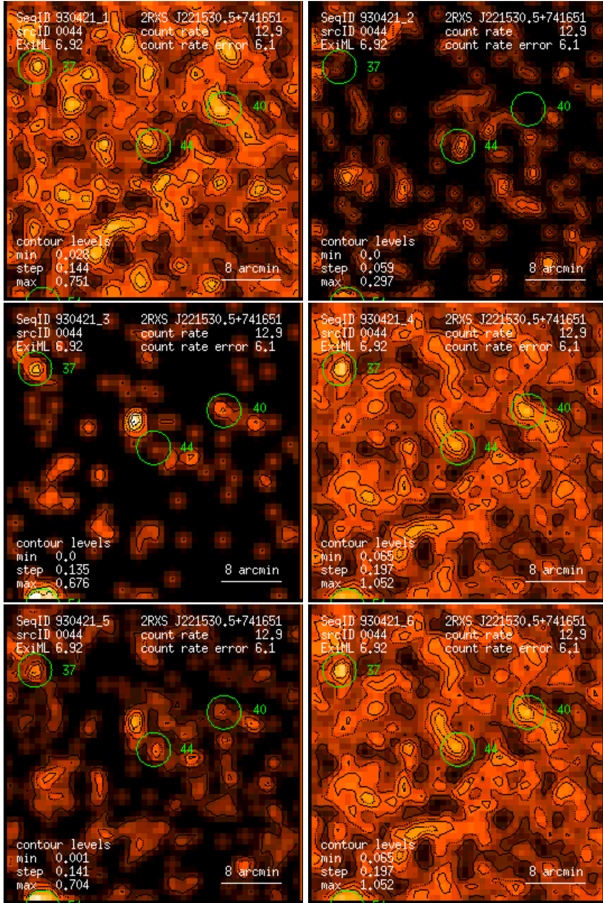
Figure 44: RASS 930421: detection 0044: band rate images, Gaussian filter: (1) PSPC channels 11 – 41, (2) 52 – 90, (3) 91 – 201, (4) 11 – 235, (5) 52 – 201, (6) 11 – 201. Broad band rates in counts/ks. Band rate contour levels in counts/ks/arcmin 2 .
