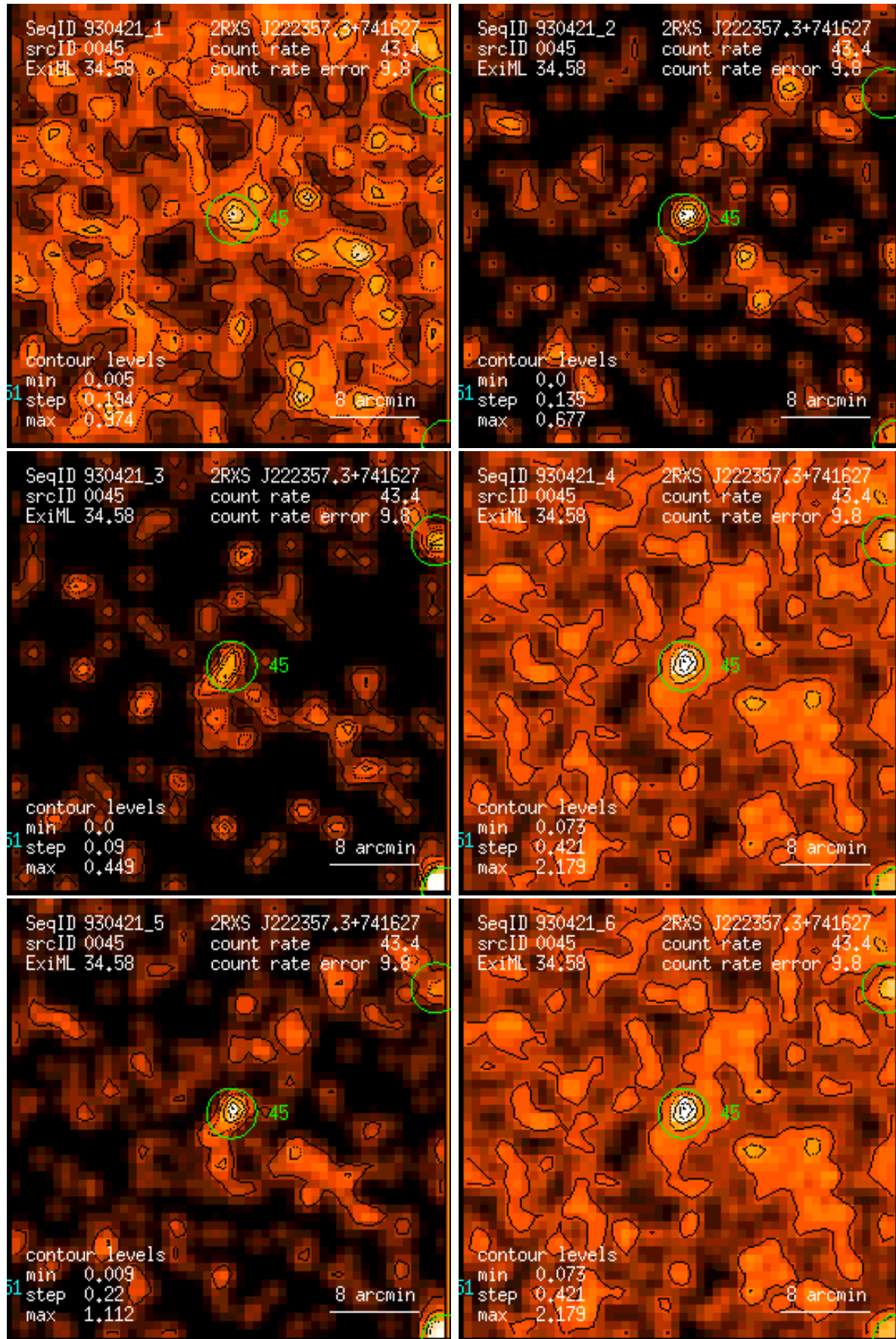
Figure 45: RASS 930421: detection 0045: band rate images, Gaussian filter: (1) PSPC channels 11 – 41, (2) 52 – 90, (3) 91 – 201, (4) 11 – 235, (5) 52 – 201, (6) 11 – 201. Broad band rates in counts/ks. Band rate contour levels in counts/ks/arcmin 2 .
