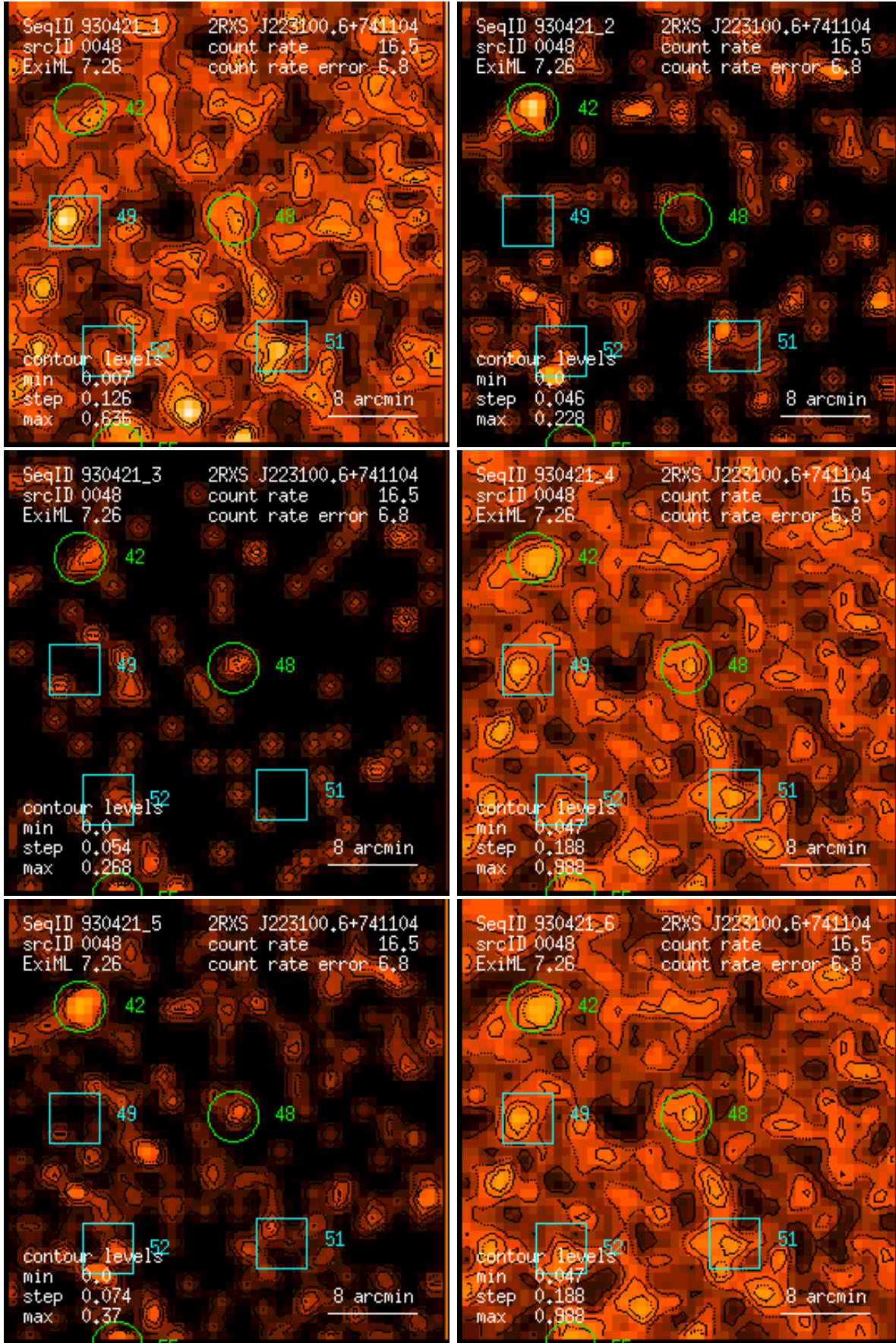
Figure 48: RASS 930421: detection 0048: band rate images, Gaussian filter: (1) PSPC channels 11 – 41, (2) 52 – 90, (3) 91 – 201, (4) 11 – 235, (5) 52 – 201, (6) 11 – 201. Broad band rates in counts/ks. Band rate contour levels in counts/ks/arcmin 2 .
