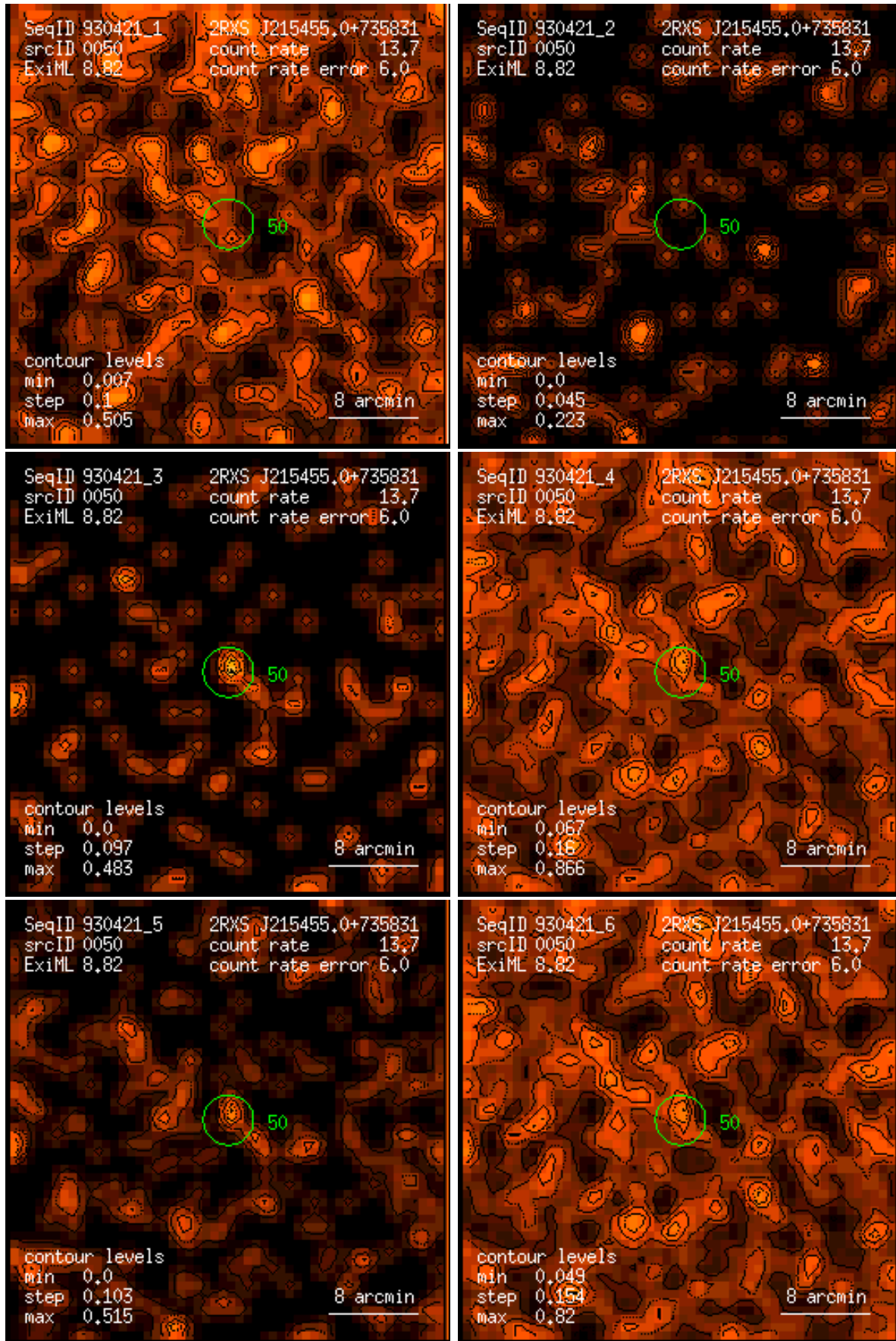
Figure 50: RASS 930421: detection 0050: band rate images, Gaussian filter: (1) PSPC channels 11 – 41, (2) 52 – 90, (3) 91 – 201, (4) 11 – 235, (5) 52 – 201, (6) 11 – 201. Broad band rates in counts/ks. Band rate contour levels in counts/ks/arcmin 2 .
