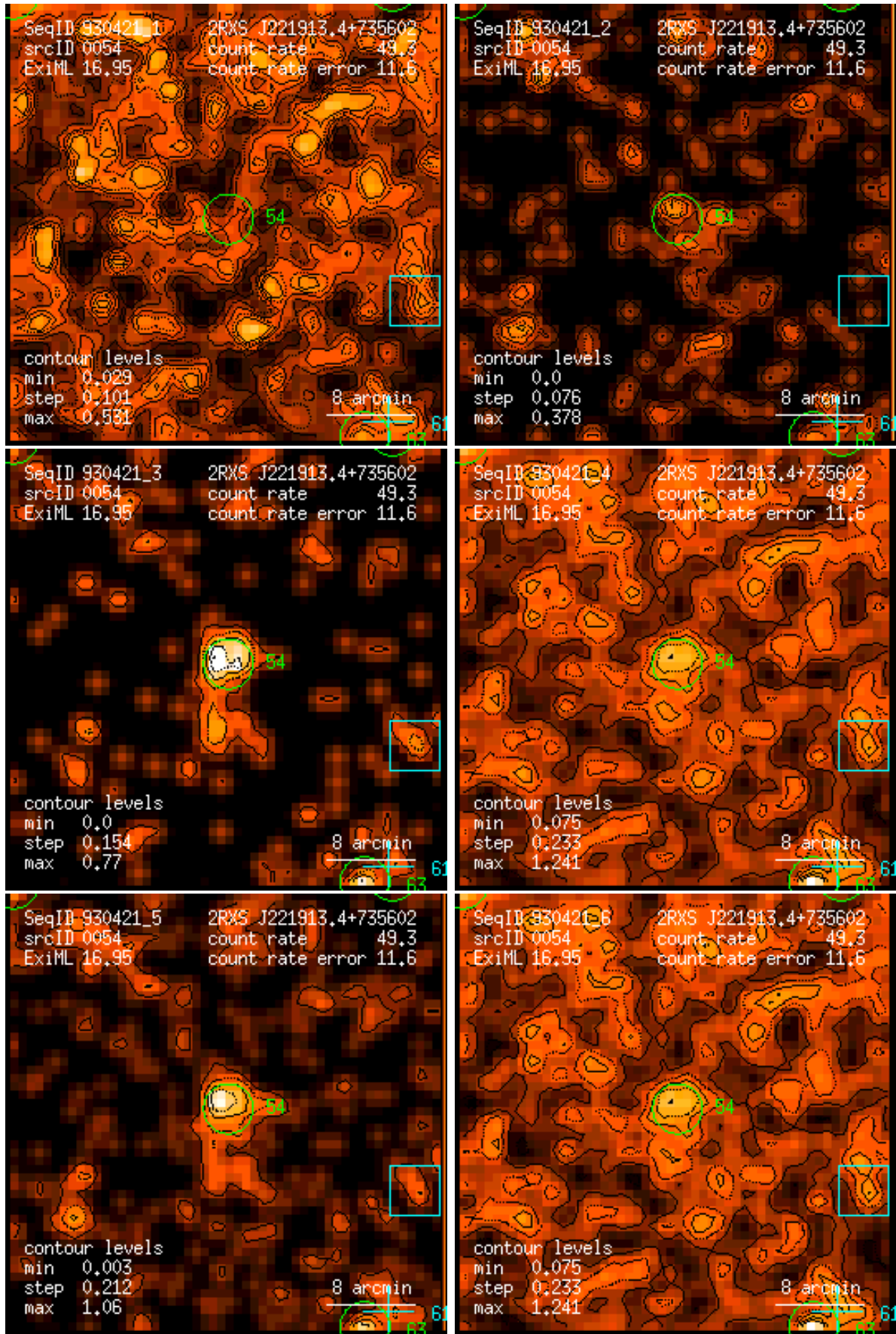
Figure 54: RASS 930421: detection 0054: band rate images, Gaussian filter: (1) PSPC channels 11 – 41, (2) 52 – 90, (3) 91 – 201, (4) 11 – 235, (5) 52 – 201, (6) 11 – 201. Broad band rates in counts/ks. Band rate contour levels in counts/ks/arcmin 2 .
