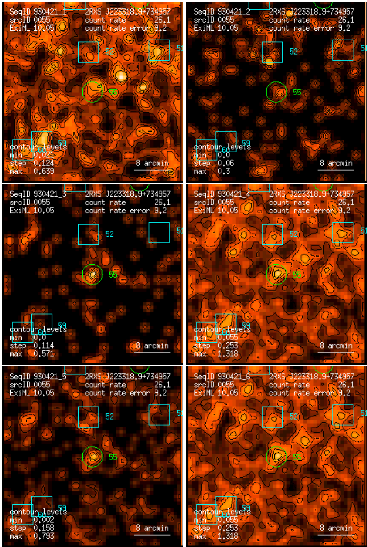
Figure 55: RASS 930421: detection 0055: band rate images, Gaussian filter: (1) PSPC channels 11 – 41, (2) 52 – 90, (3) 91 – 201, (4) 11 – 235, (5) 52 – 201, (6) 11 – 201. Broad band rates in counts/ks. Band rate contour levels in counts/ks/arcmin 2 .
