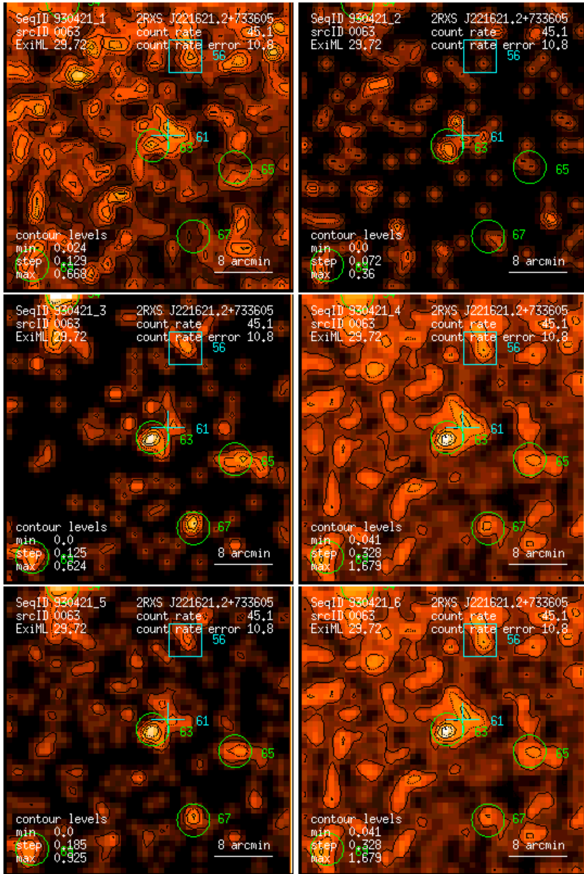
Figure 63: RASS 930421: detection 0063: band rate images, Gaussian filter: (1) PSPC channels 11 – 41, (2) 52 – 90, (3) 91 – 201, (4) 11 – 235, (5) 52 – 201, (6) 11 – 201. Broad band rates in counts/ks. Band rate contour levels in counts/ks/arcmin 2 .
