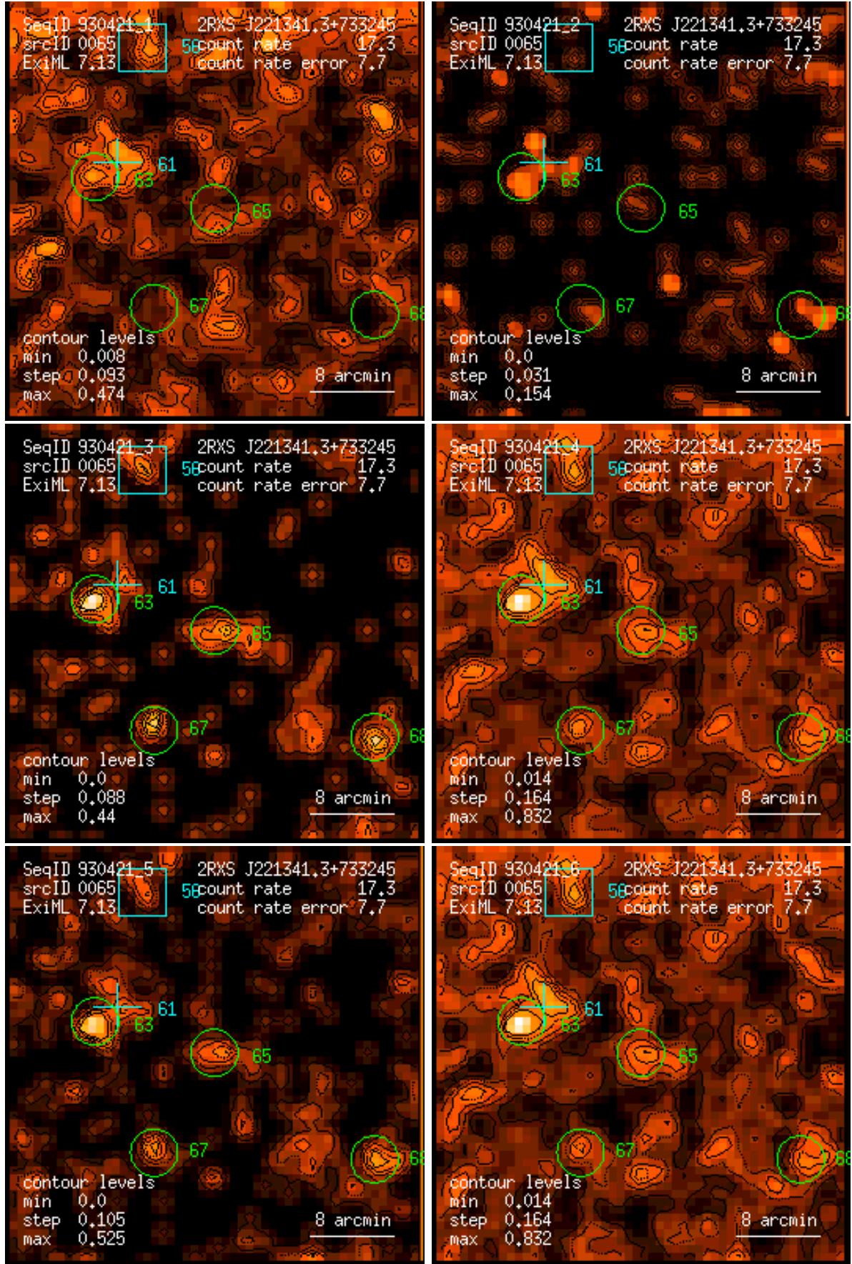
Figure 65: RASS 930421: detection 0065: band rate images, Gaussian filter: (1) PSPC channels 11 – 41, (2) 52 – 90, (3) 91 – 201, (4) 11 – 235, (5) 52 – 201, (6) 11 – 201. Broad band rates in counts/ks. Band rate contour levels in counts/ks/arcmin 2 .
