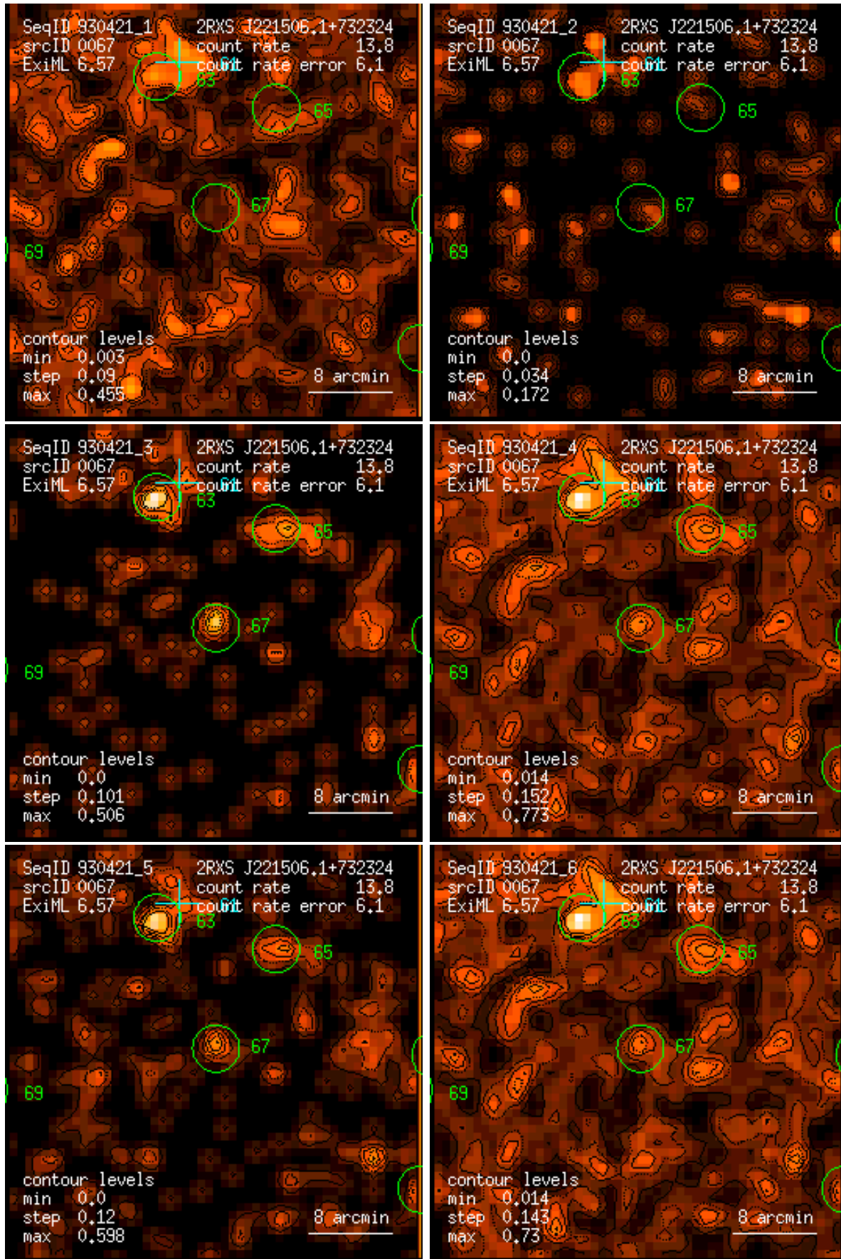
Figure 67: RASS 930421: detection 0067: band rate images, Gaussian filter: (1) PSPC channels 11 – 41, (2) 52 – 90, (3) 91 – 201, (4) 11 – 235, (5) 52 – 201, (6) 11 – 201. Broad band rates in counts/ks. Band rate contour levels in counts/ks/arcmin 2 .
