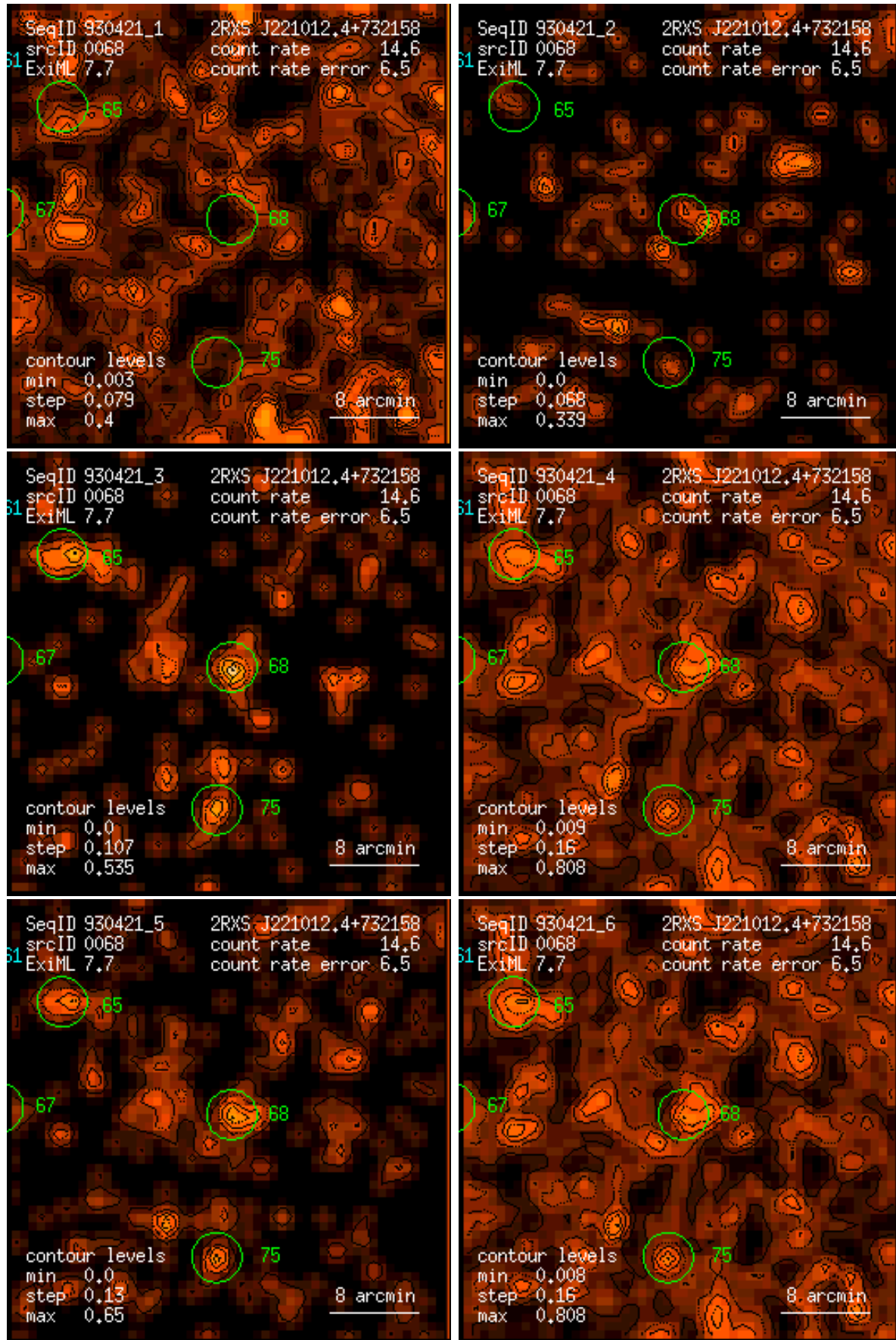
Figure 68: RASS 930421: detection 0068: band rate images, Gaussian filter: (1) PSPC channels 11 – 41, (2) 52 – 90, (3) 91 – 201, (4) 11 – 235, (5) 52 – 201, (6) 11 – 201. Broad band rates in counts/ks. Band rate contour levels in counts/ks/arcmin 2 .
