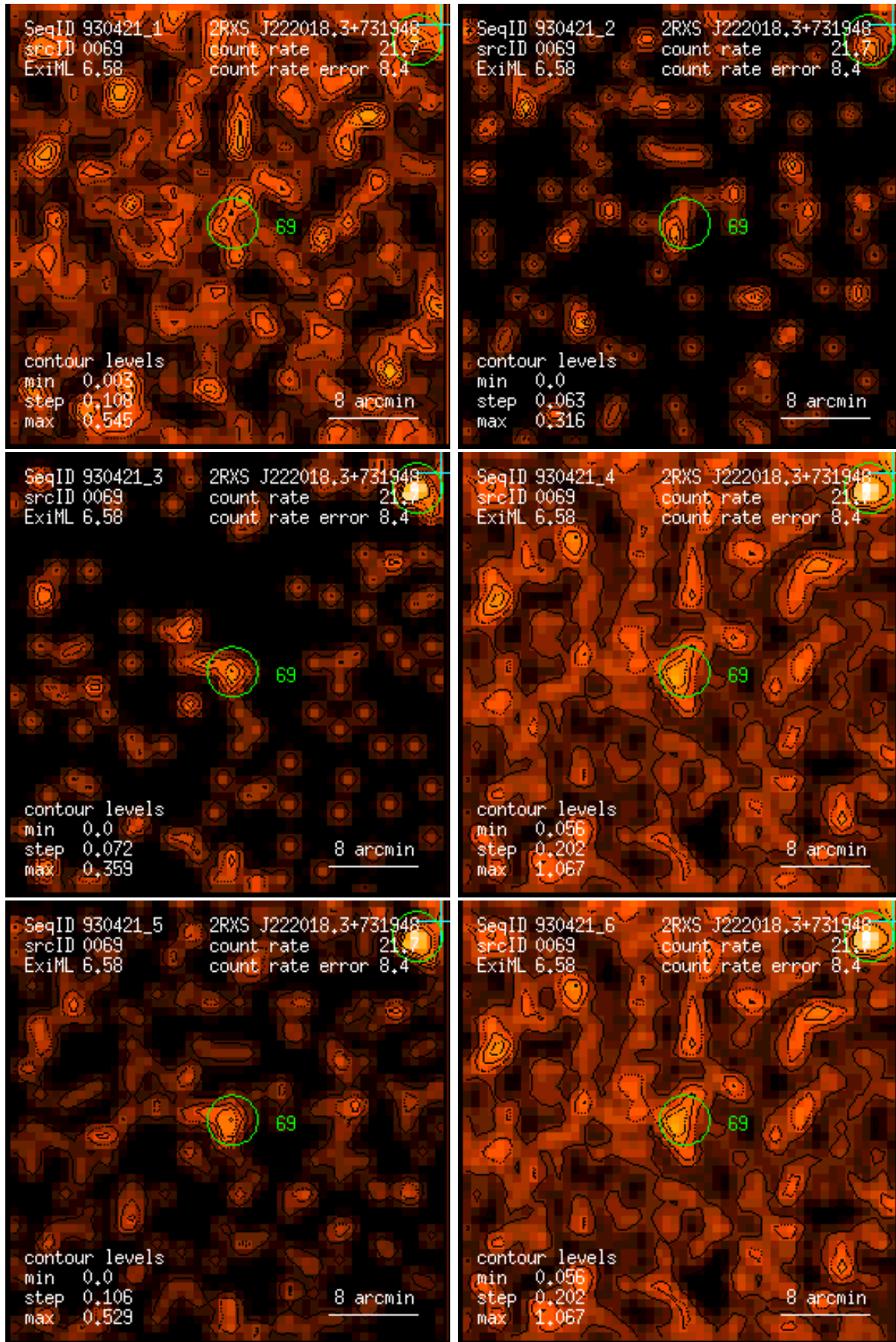
Figure 69: RASS 930421: detection 0069: band rate images, Gaussian filter: (1) PSPC channels 11 – 41, (2) 52 – 90, (3) 91 – 201, (4) 11 – 235, (5) 52 – 201, (6) 11 – 201. Broad band rates in counts/ks. Band rate contour levels in counts/ks/arcmin 2 .
