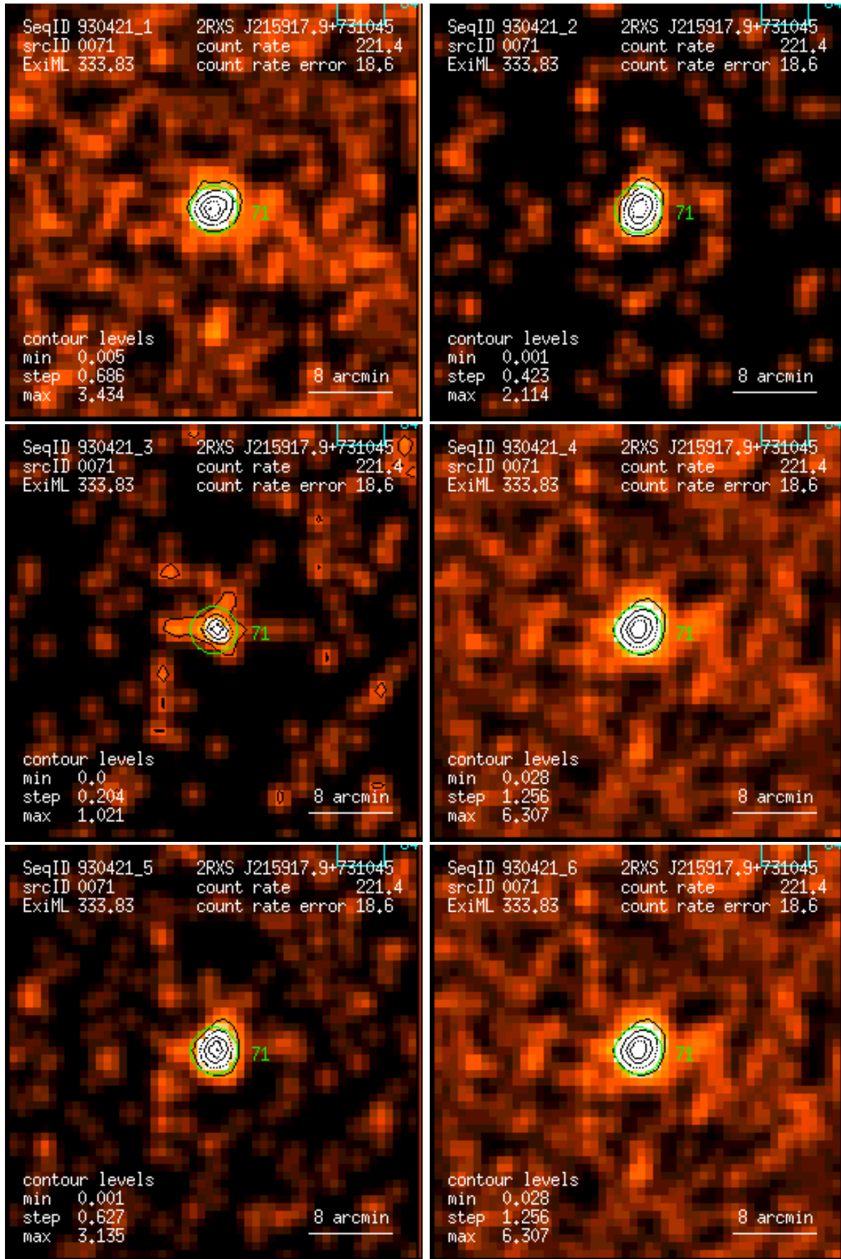
Figure 71: RASS 930421: detection 0071: band rate images, Gaussian filter: (1) PSPC channels 11 – 41, (2) 52 – 90, (3) 91 – 201, (4) 11 – 235, (5) 52 – 201, (6) 11 – 201. Broad band rates in counts/ks. Band rate contour levels in counts/ks/arcmin 2 .
