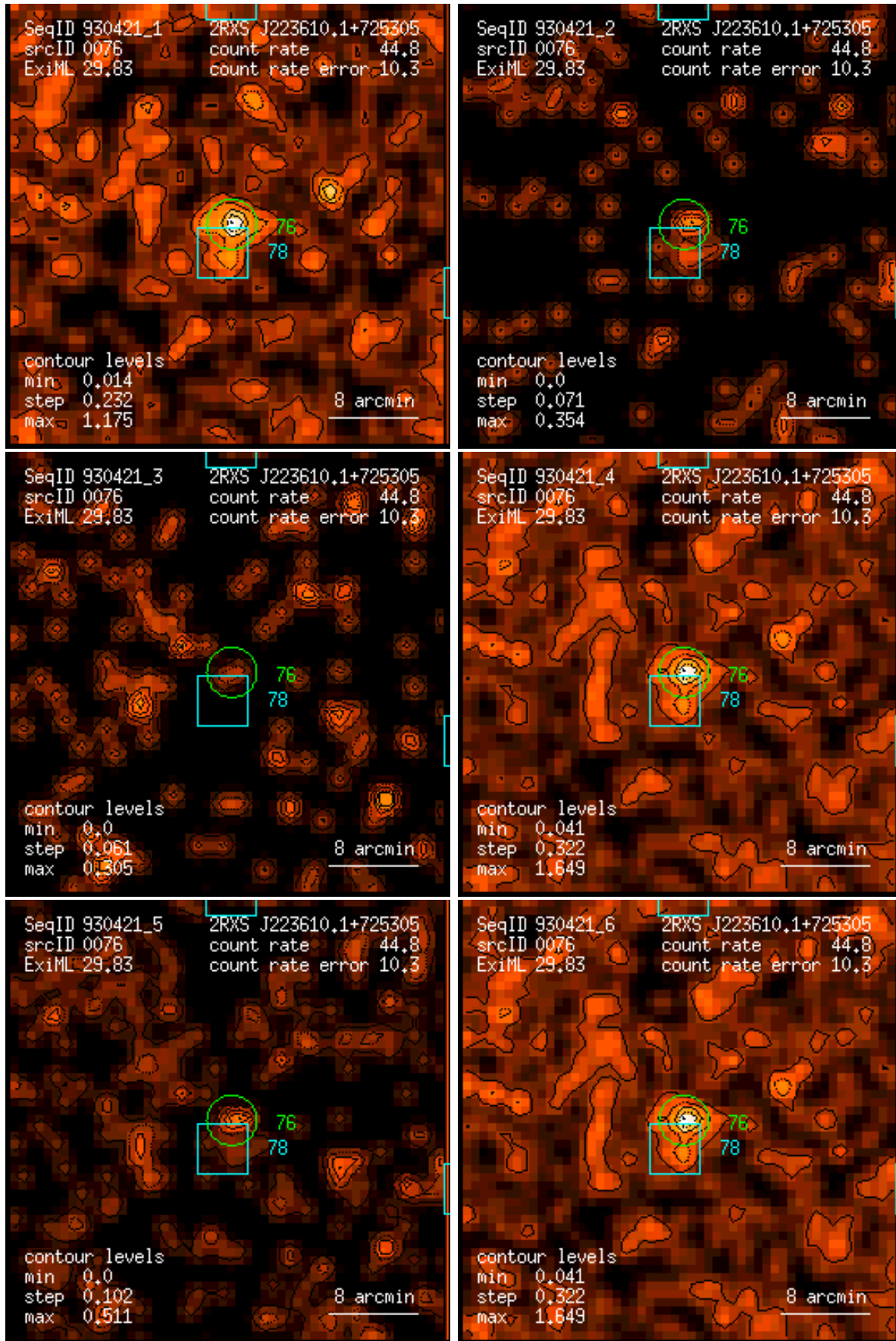
Figure 76: RASS 930421: detection 0076: band rate images, Gaussian filter: (1) PSPC channels 11 – 41, (2) 52 – 90, (3) 91 – 201, (4) 11 – 235, (5) 52 – 201, (6) 11 – 201. Broad band rates in counts/ks. Band rate contour levels in counts/ks/arcmin 2 .
