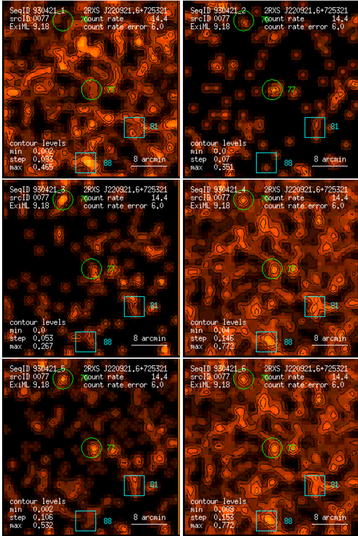
Figure 77: RASS 930421: detection 0077: band rate images, Gaussian filter: (1) PSPC channels 11 – 41, (2) 52 – 90, (3) 91 – 201, (4) 11 – 235, (5) 52 – 201, (6) 11 – 201. Broad band rates in counts/ks. Band rate contour levels in counts/ks/arcmin 2 .
