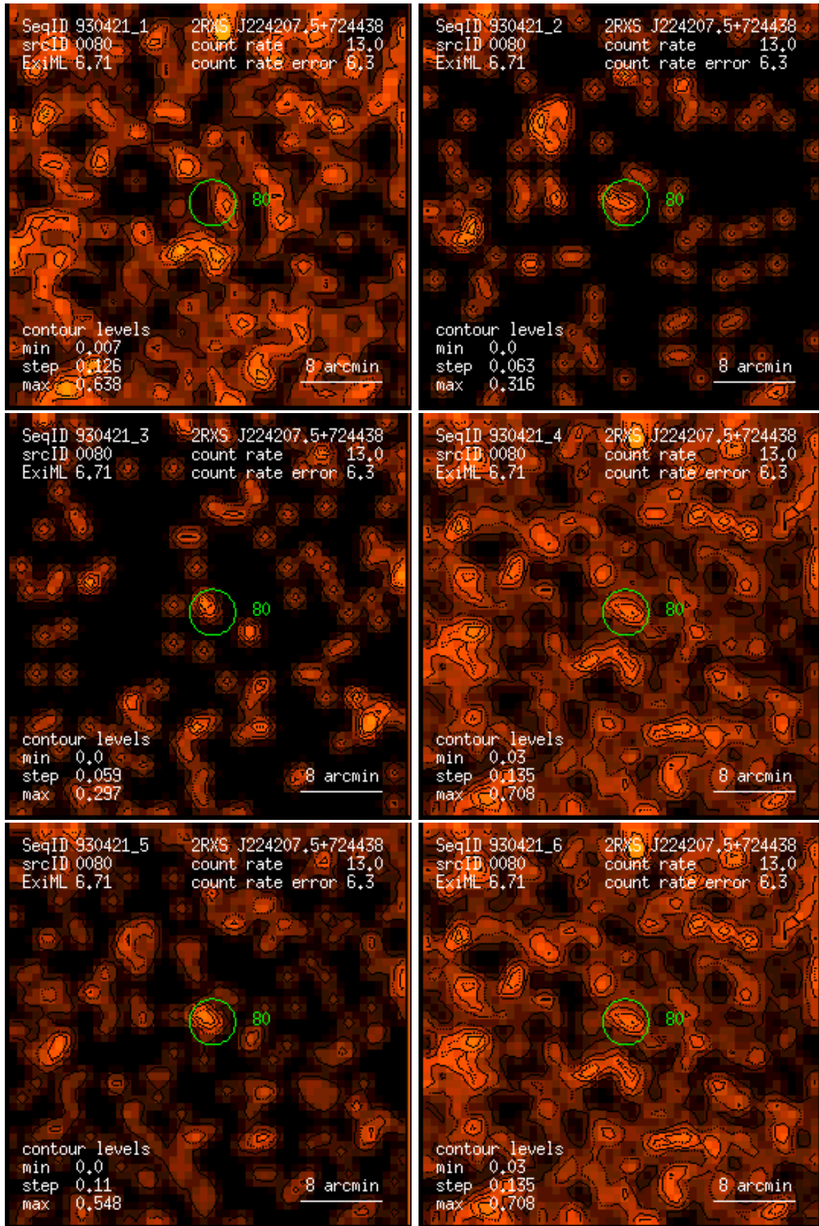
Figure 80: RASS 930421: detection 0080: band rate images, Gaussian filter: (1) PSPC channels 11 – 41, (2) 52 – 90, (3) 91 – 201, (4) 11 – 235, (5) 52 – 201, (6) 11 – 201. Broad band rates in counts/ks. Band rate contour levels in counts/ks/arcmin 2 .
