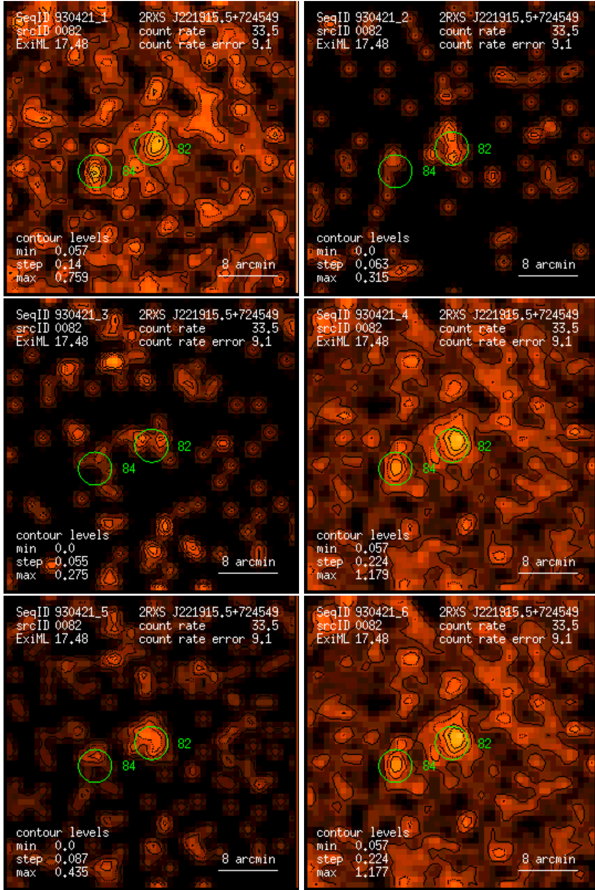
Figure 82: RASS 930421: detection 0082: band rate images, Gaussian filter: (1) PSPC channels 11 – 41, (2) 52 – 90, (3) 91 – 201, (4) 11 – 235, (5) 52 – 201, (6) 11 – 201. Broad band rates in counts/ks. Band rate contour levels in counts/ks/arcmin 2 .
