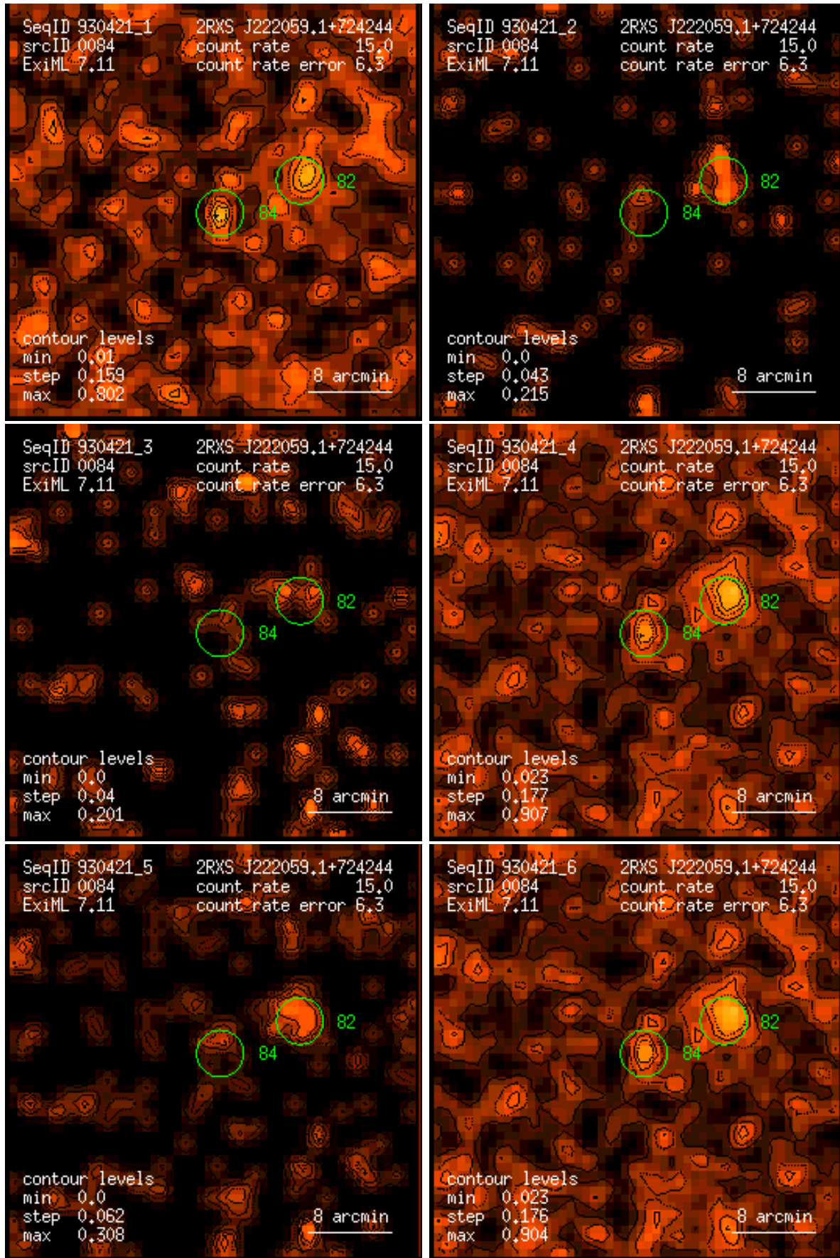
Figure 84: RASS 930421: detection 0084: band rate images, Gaussian filter: (1) PSPC channels 11 – 41, (2) 52 – 90, (3) 91 – 201, (4) 11 – 235, (5) 52 – 201, (6) 11 – 201. Broad band rates in counts/ks. Band rate contour levels in counts/ks/arcmin 2 .
