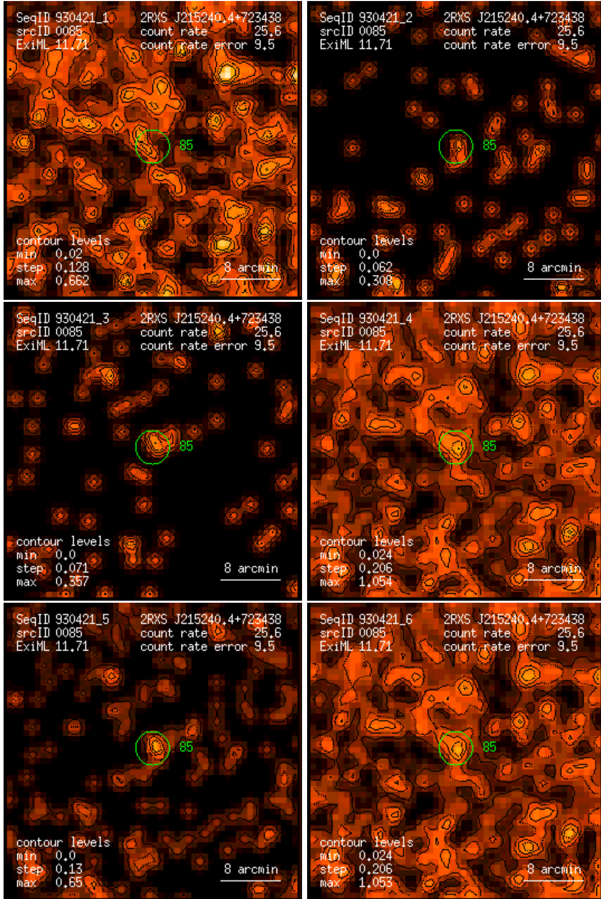
Figure 85: RASS 930421: detection 0085: band rate images, Gaussian filter: (1) PSPC channels 11 – 41, (2) 52 – 90, (3) 91 – 201, (4) 11 – 235, (5) 52 – 201, (6) 11 – 201. Broad band rates in counts/ks. Band rate contour levels in counts/ks/arcmin 2 .
