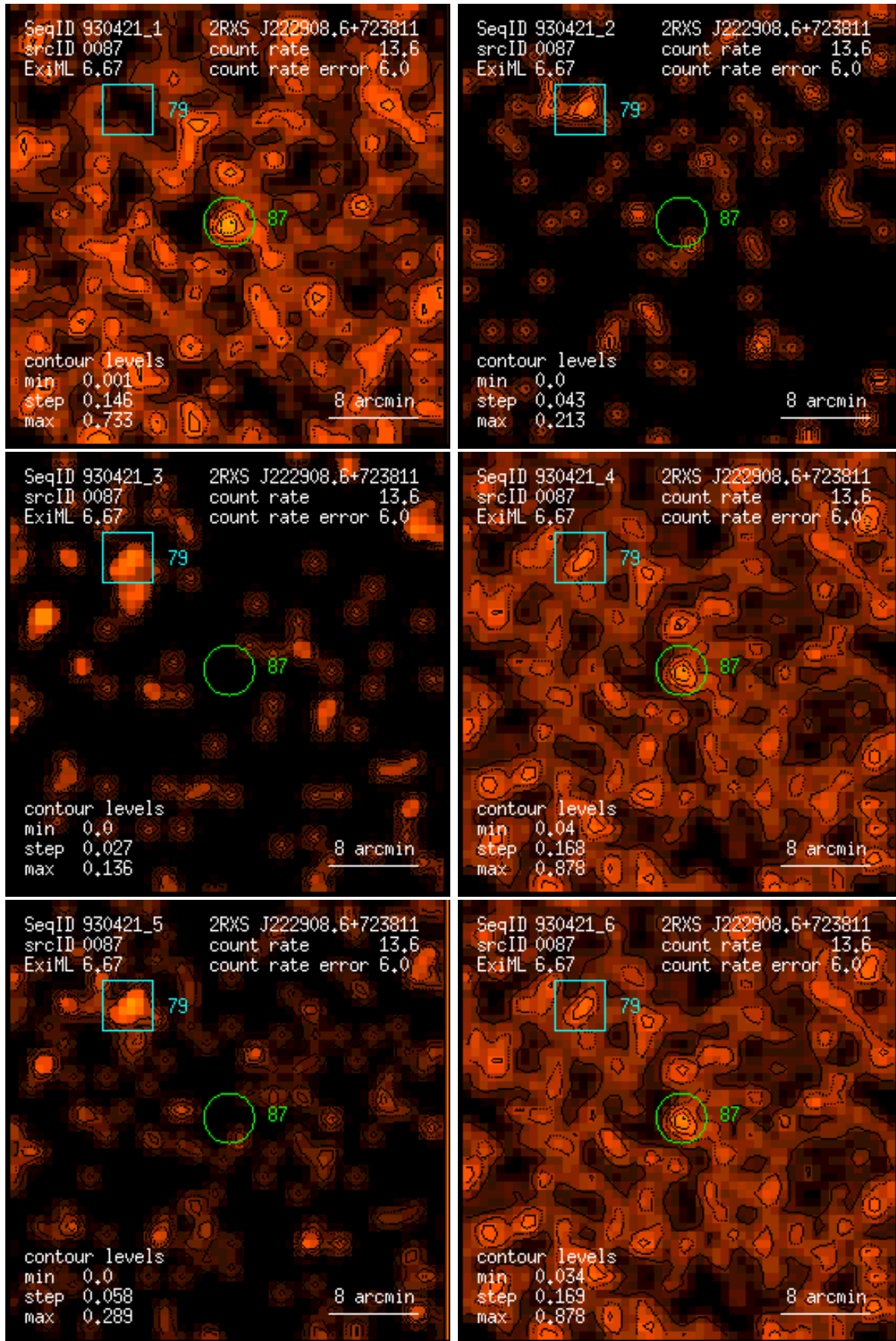
Figure 87: RASS 930421: detection 0087: band rate images, Gaussian filter: (1) PSPC channels 11 – 41, (2) 52 – 90, (3) 91 – 201, (4) 11 – 235, (5) 52 – 201, (6) 11 – 201. Broad band rates in counts/ks. Band rate contour levels in counts/ks/arcmin 2 .
