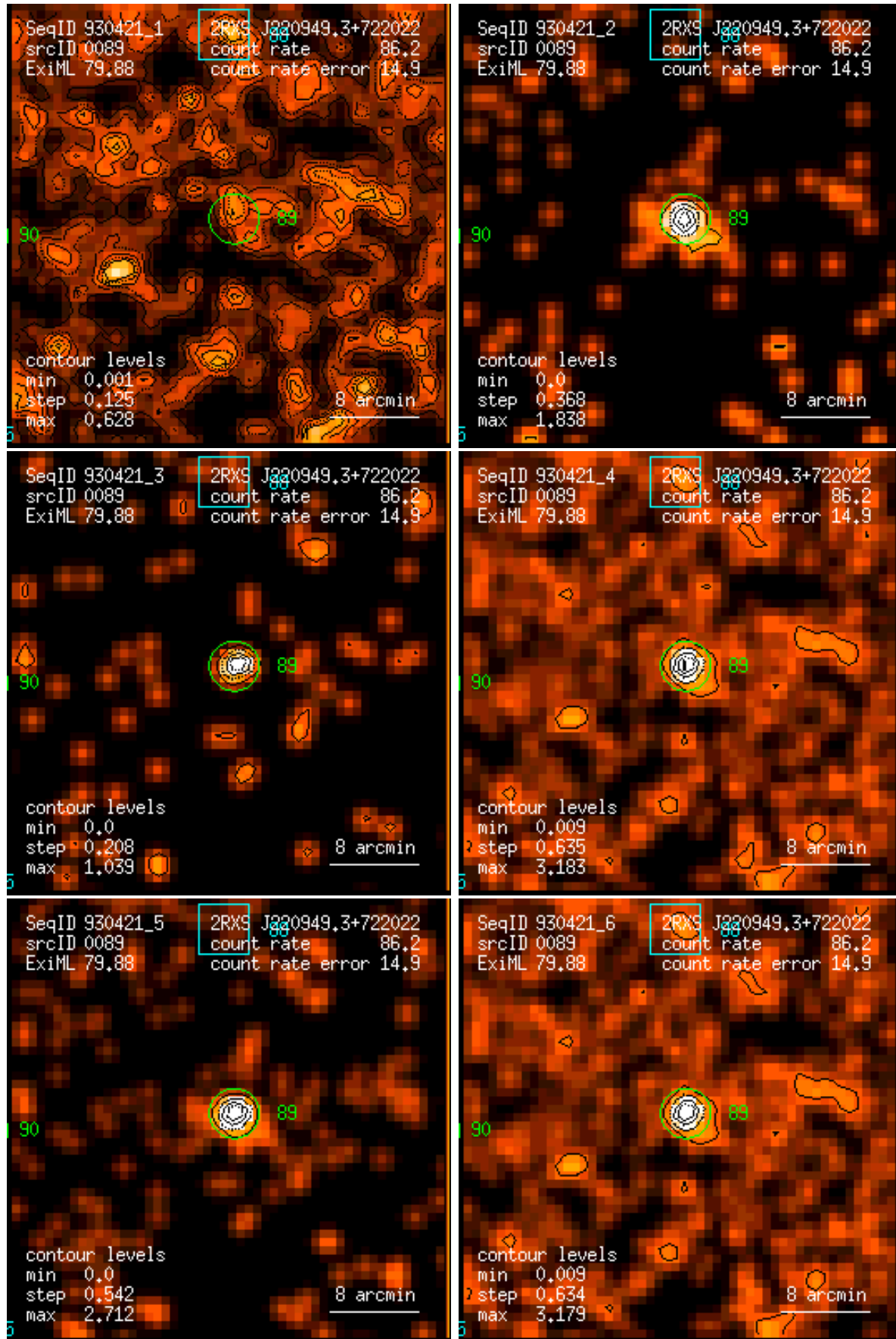
Figure 89: RASS 930421: detection 0089: band rate images, Gaussian filter: (1) PSPC channels 11 – 41, (2) 52 – 90, (3) 91 – 201, (4) 11 – 235, (5) 52 – 201, (6) 11 – 201. Broad band rates in counts/ks. Band rate contour levels in counts/ks/arcmin 2 .
