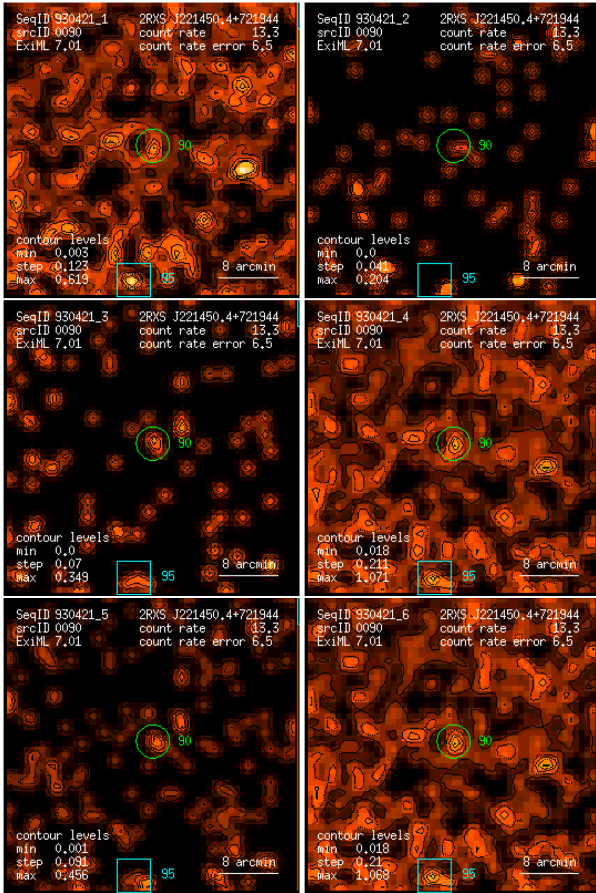
Figure 90: RASS 930421: detection 0090: band rate images, Gaussian filter: (1) PSPC channels 11 – 41, (2) 52 – 90, (3) 91 – 201, (4) 11 – 235, (5) 52 – 201, (6) 11 – 201. Broad band rates in counts/ks. Band rate contour levels in counts/ks/arcmin 2 .
