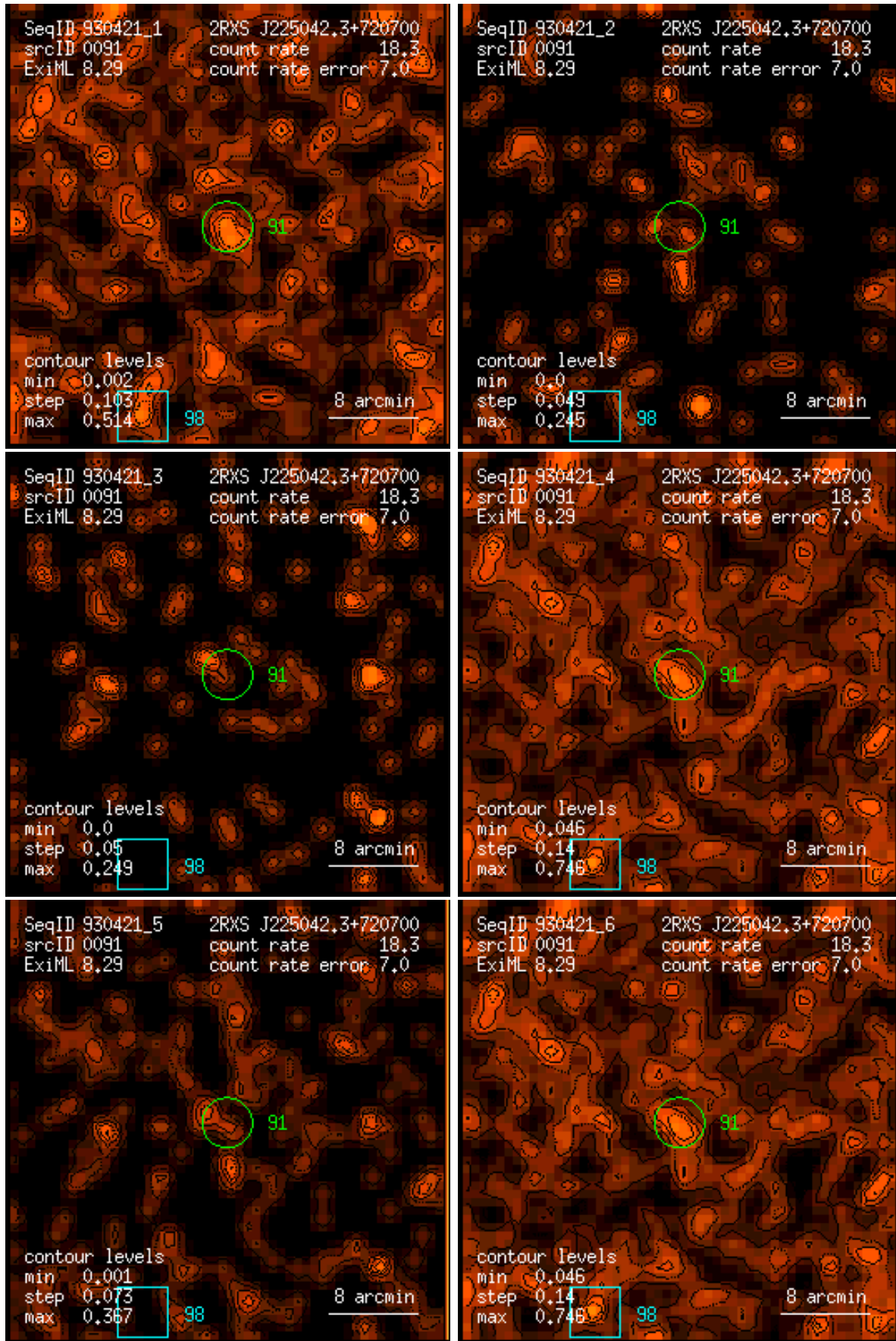
Figure 91: RASS 930421: detection 0091: band rate images, Gaussian filter: (1) PSPC channels 11 – 41, (2) 52 – 90, (3) 91 – 201, (4) 11 – 235, (5) 52 – 201, (6) 11 – 201. Broad band rates in counts/ks. Band rate contour levels in counts/ks/arcmin 2 .
