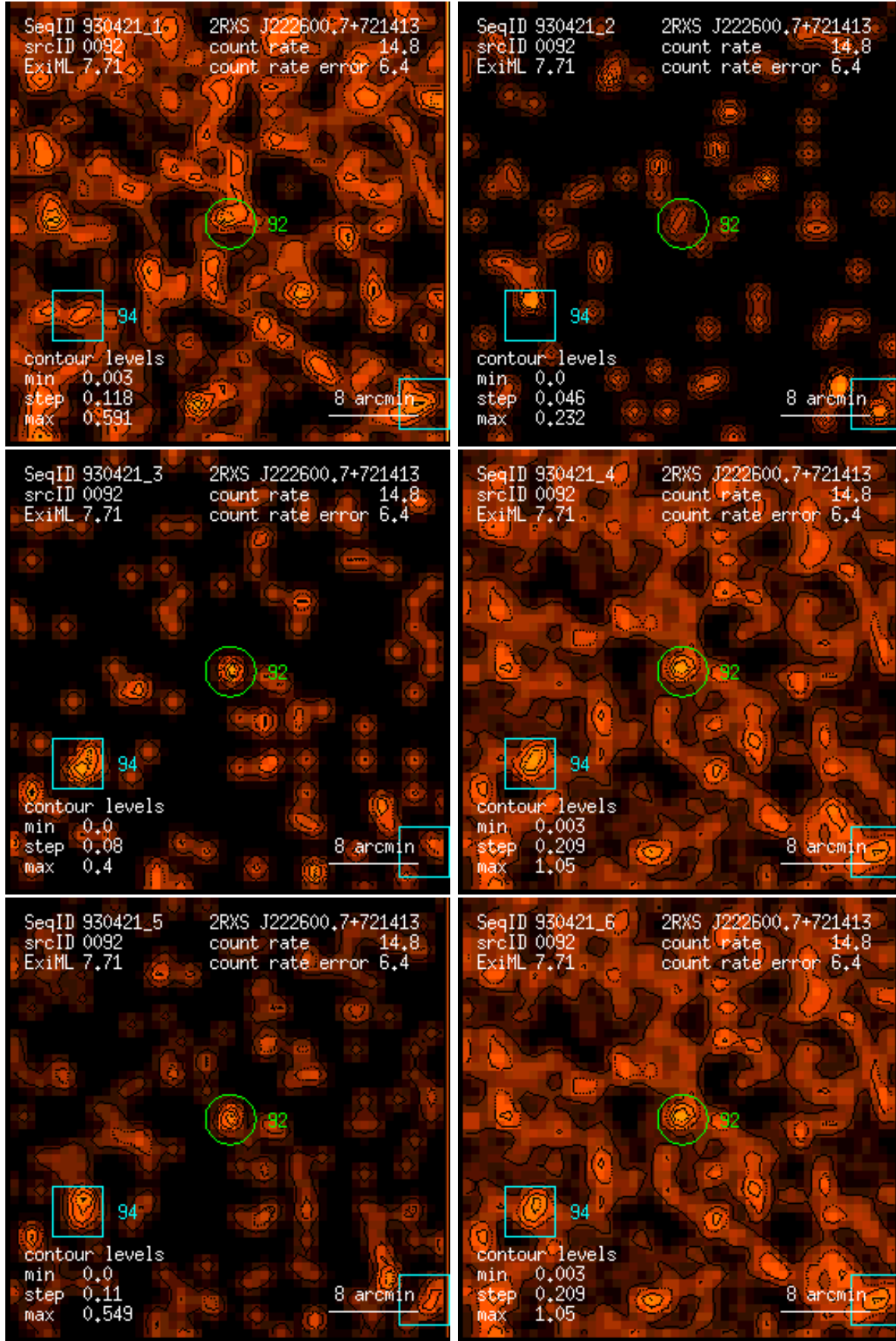
Figure 92: RASS 930421: detection 0092: band rate images, Gaussian filter: (1) PSPC channels 11 – 41, (2) 52 – 90, (3) 91 – 201, (4) 11 – 235, (5) 52 – 201, (6) 11 – 201. Broad band rates in counts/ks. Band rate contour levels in counts/ks/arcmin 2 .
