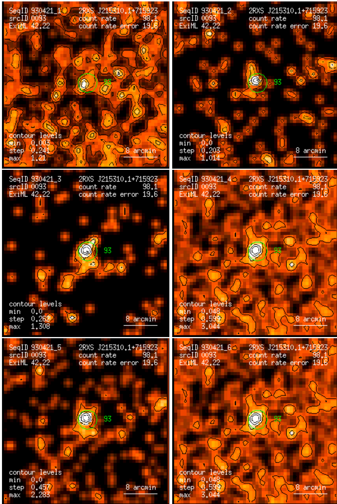
Figure 93: RASS 930421: detection 0093: band rate images, Gaussian filter: (1) PSPC channels 11 – 41, (2) 52 – 90, (3) 91 – 201, (4) 11 – 235, (5) 52 – 201, (6) 11 – 201. Broad band rates in counts/ks. Band rate contour levels in counts/ks/arcmin 2 .
