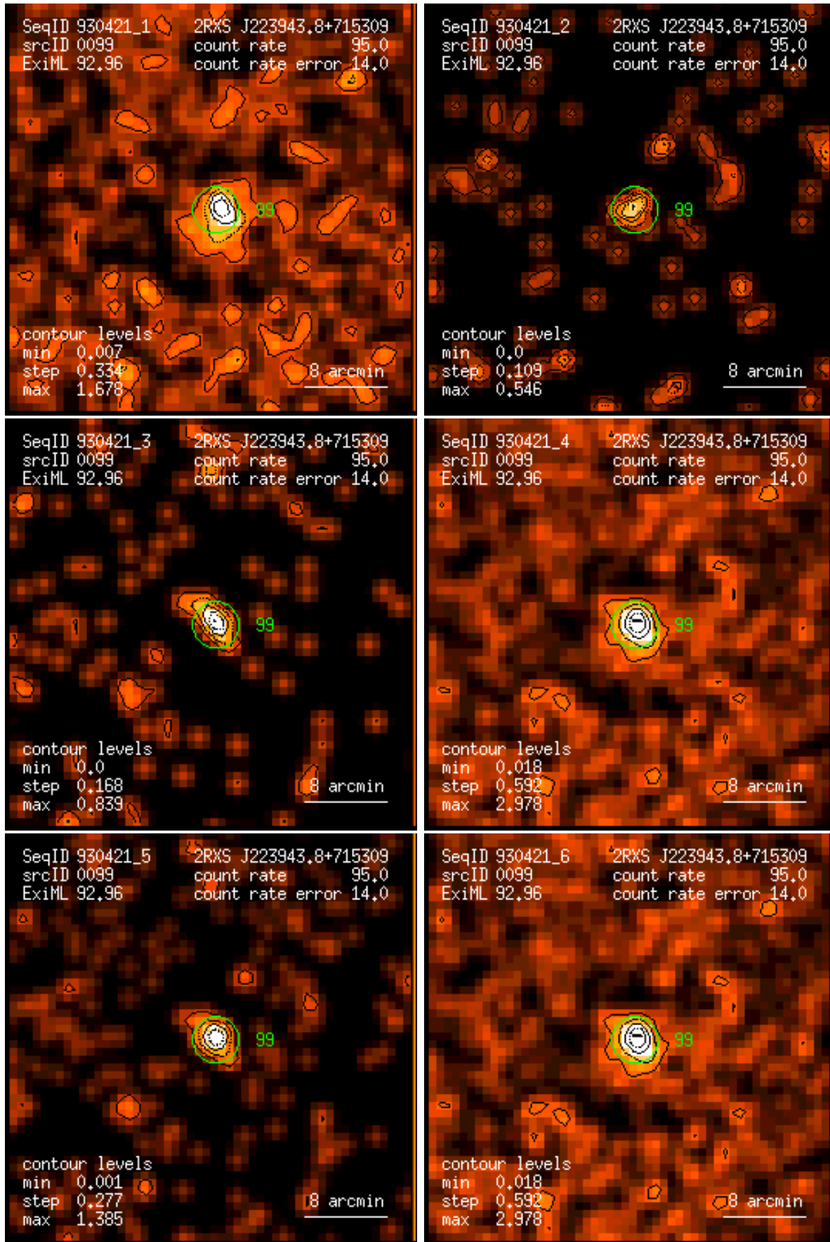
Figure 99: RASS 930421: detection 0099: band rate images, Gaussian filter: (1) PSPC channels 11 – 41, (2) 52 – 90, (3) 91 – 201, (4) 11 – 235, (5) 52 – 201, (6) 11 – 201. Broad band rates in counts/ks. Band rate contour levels in counts/ks/arcmin 2 .
