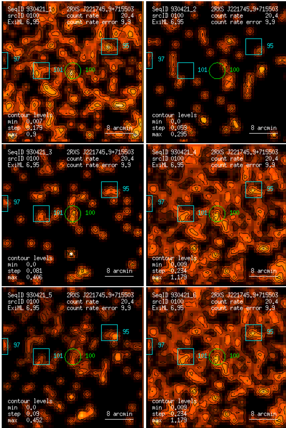
Figure 100: RASS 930421: detection 0100: band rate images, Gaussian filter: (1) PSPC channels 11 – 41, (2) 52 – 90, (3) 91 – 201, (4) 11 – 235, (5) 52 – 201, (6) 11 – 201. Broad band rates in counts/ks. Band rate contour levels in counts/ks/arcmin 2 .
