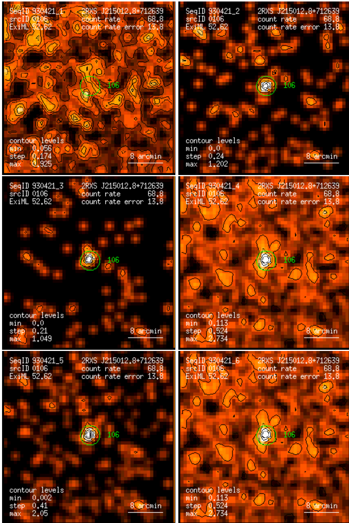
Figure 106: RASS 930421: detection 0106: band rate images, Gaussian filter: (1) PSPC channels 11 – 41, (2) 52 – 90, (3) 91 – 201, (4) 11 – 235, (5) 52 – 201, (6) 11 – 201. Broad band rates in counts/ks. Band rate contour levels in counts/ks/arcmin 2 .
