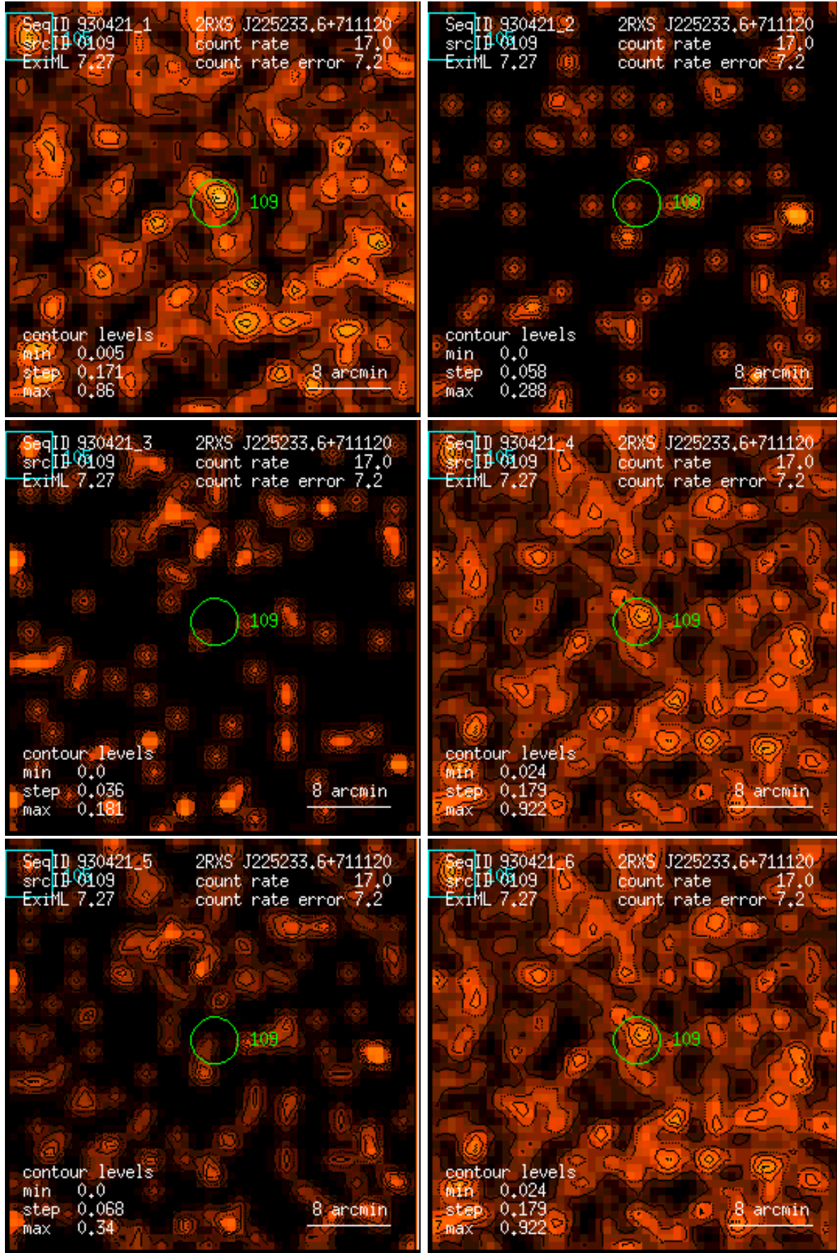
Figure 109: RASS 930421: detection 0109: band rate images, Gaussian filter: (1) PSPC channels 11 – 41, (2) 52 – 90, (3) 91 – 201, (4) 11 – 235, (5) 52 – 201, (6) 11 – 201. Broad band rates in counts/ks. Band rate contour levels in counts/ks/arcmin 2 .
