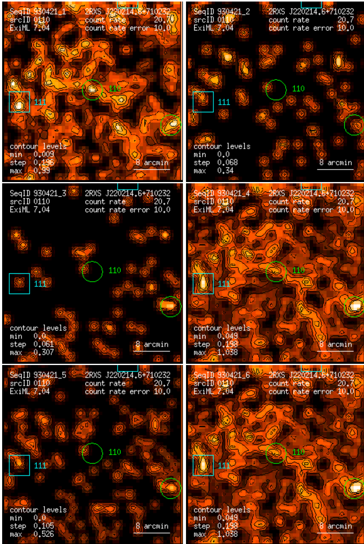
Figure 110: RASS 930421: detection 0110: band rate images, Gaussian filter: (1) PSPC channels 11 – 41, (2) 52 – 90, (3) 91 – 201, (4) 11 – 235, (5) 52 – 201, (6) 11 – 201. Broad band rates in counts/ks. Band rate contour levels in counts/ks/arcmin 2 .
