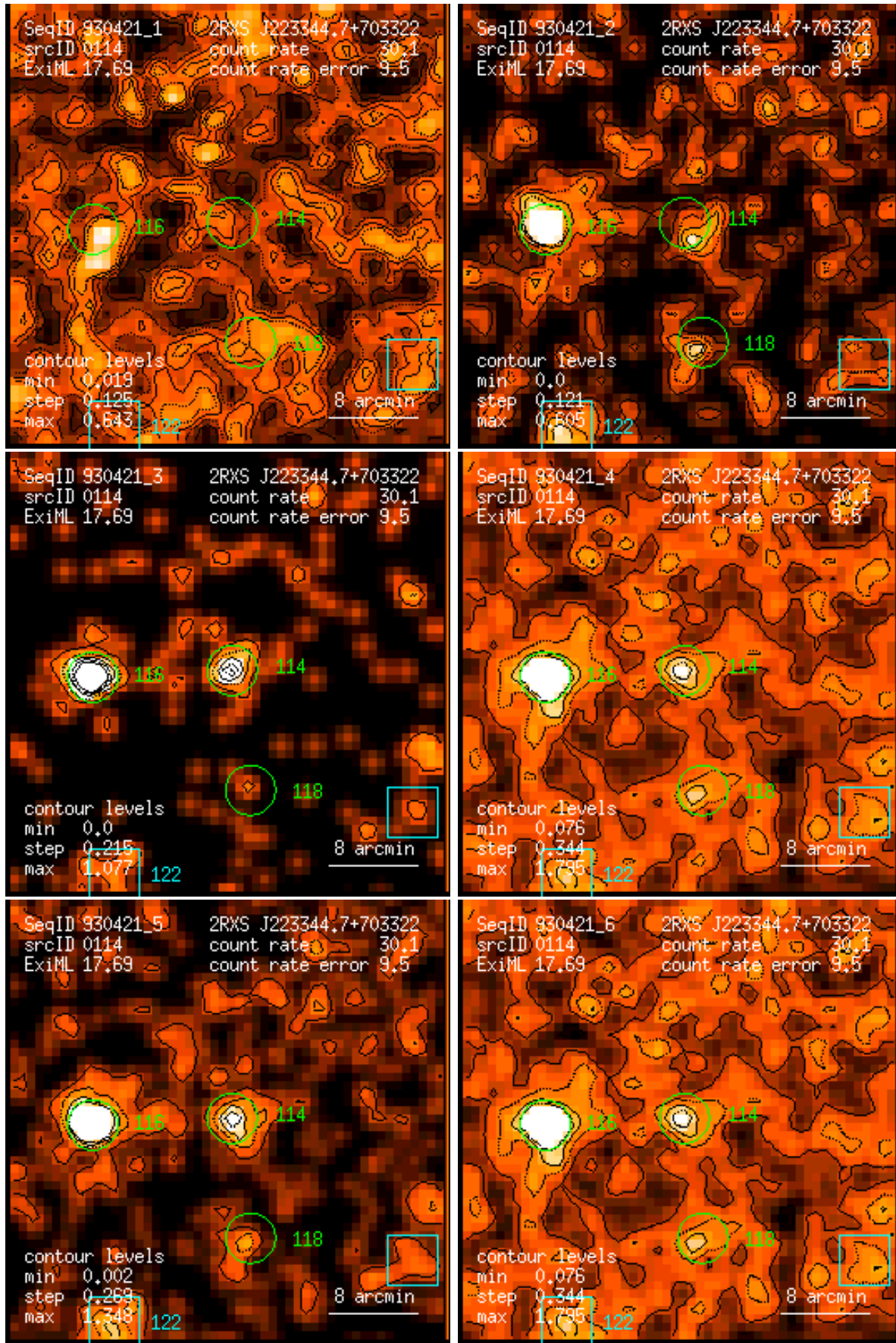
Figure 114: RASS 930421: detection 0114: band rate images, Gaussian filter: (1) PSPC channels 11 – 41, (2) 52 – 90, (3) 91 – 201, (4) 11 – 235, (5) 52 – 201, (6) 11 – 201. Broad band rates in counts/ks. Band rate contour levels in counts/ks/arcmin 2 .
