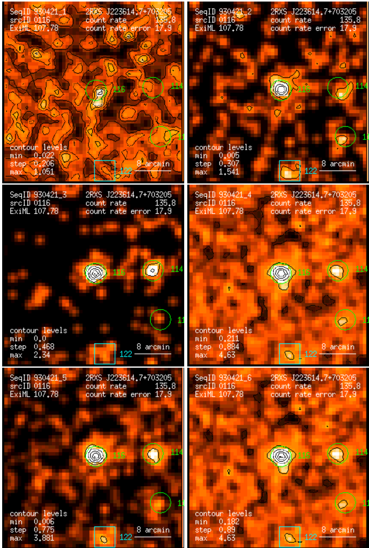
Figure 116: RASS 930421: detection 0116: band rate images, Gaussian filter: (1) PSPC channels 11 – 41, (2) 52 – 90, (3) 91 – 201, (4) 11 – 235, (5) 52 – 201, (6) 11 – 201. Broad band rates in counts/ks. Band rate contour levels in counts/ks/arcmin 2 .
