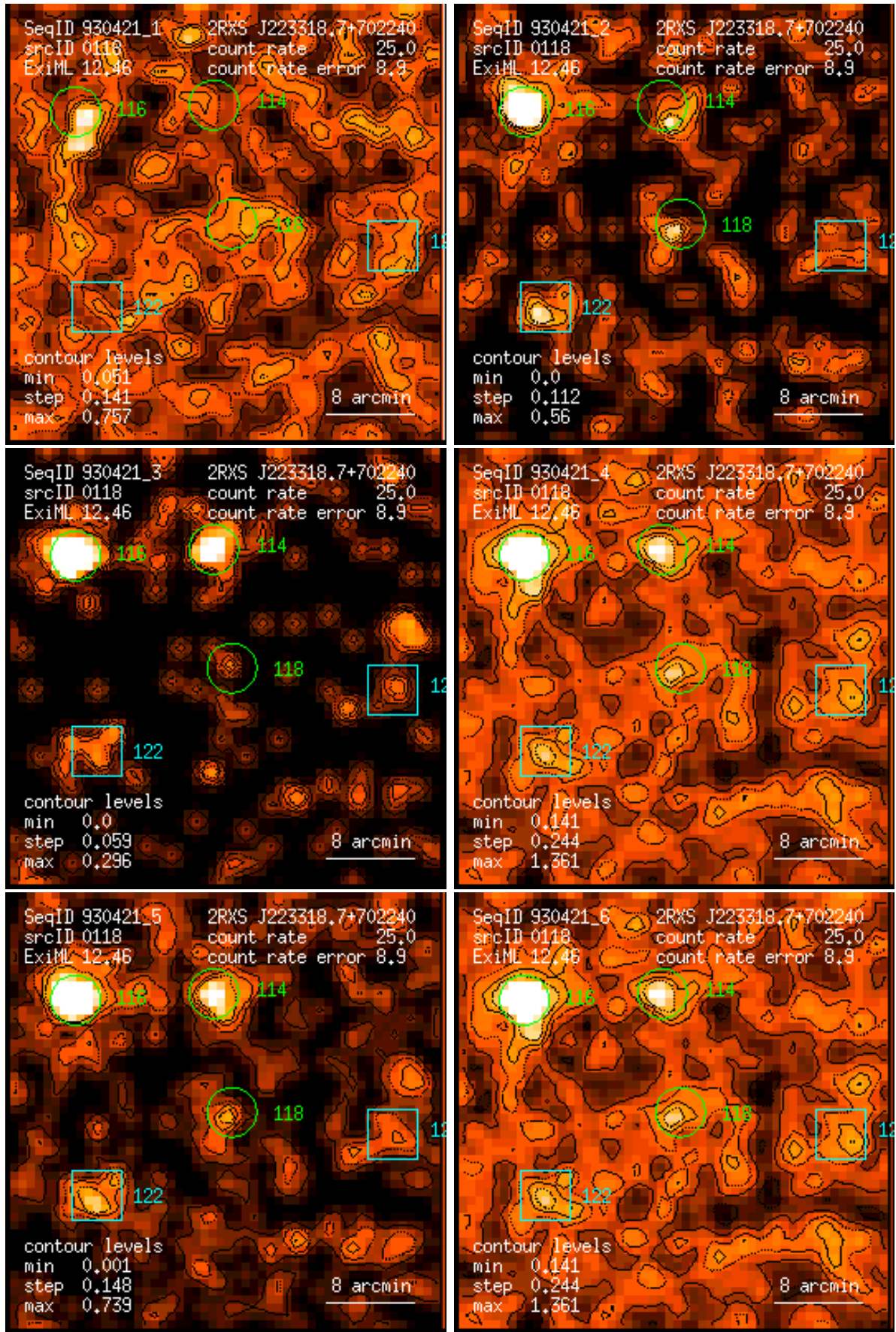
Figure 118: RASS 930421: detection 0118: band rate images, Gaussian filter: (1) PSPC channels 11 – 41, (2) 52 – 90, (3) 91 – 201, (4) 11 – 235, (5) 52 – 201, (6) 11 – 201. Broad band rates in counts/ks. Band rate contour levels in counts/ks/arcmin 2 .
