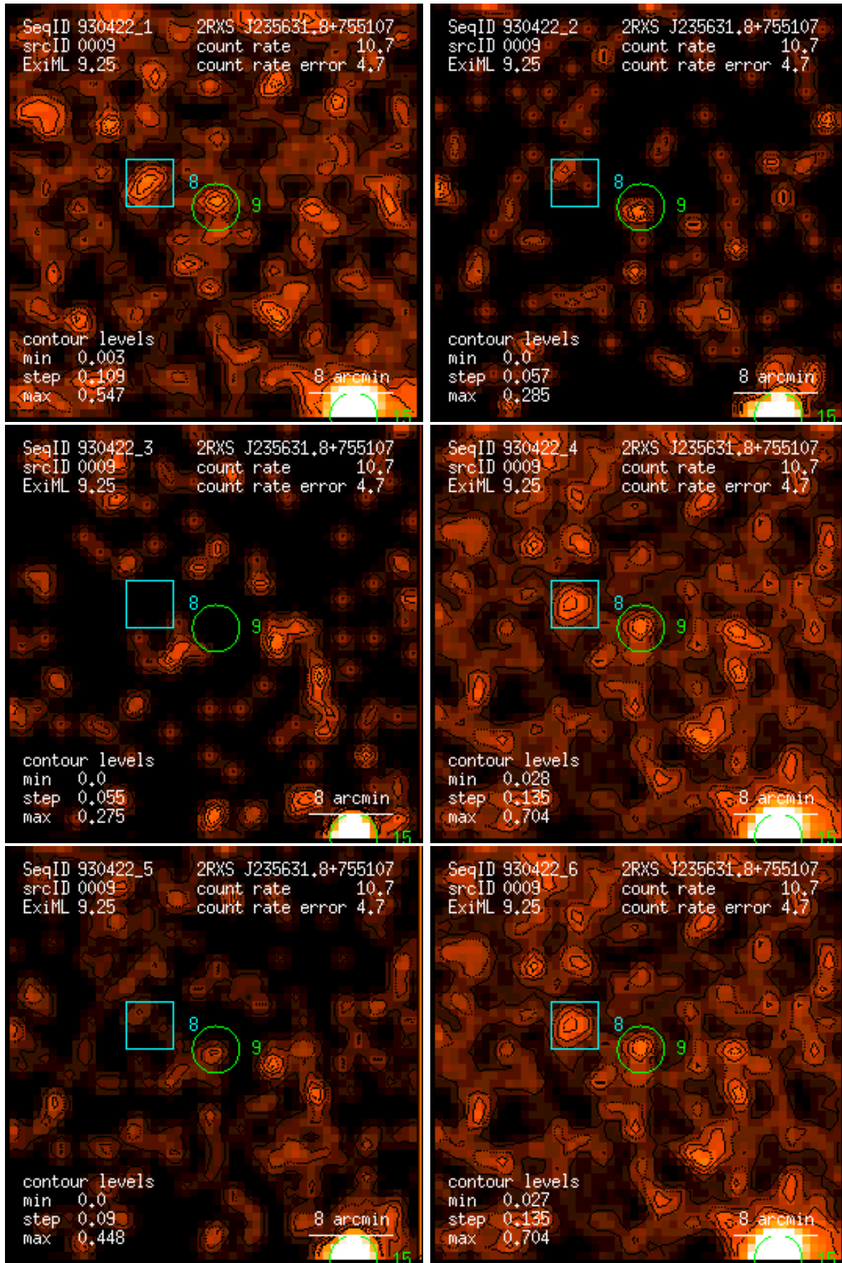
Figure 9: RASS 930422: detection 0009: band rate images, Gaussian filter: (1) PSPC channels 11 – 41, (2) 52 – 90, (3) 91 – 201, (4) 11 – 235, (5) 52 – 201, (6) 11 – 201. Broad band rates in counts/ks. Band rate contour levels in counts/ks/arcmin 2 .
