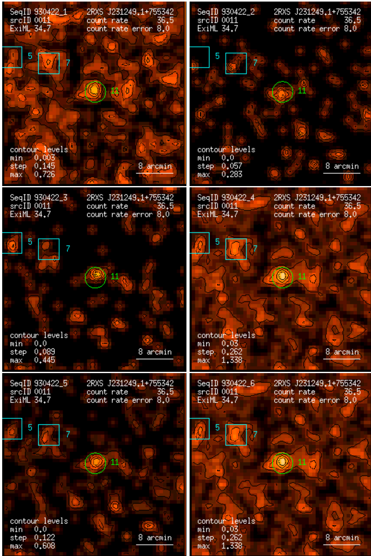
Figure 11: RASS 930422: detection 0011: band rate images, Gaussian filter: (1) PSPC channels 11 – 41, (2) 52 – 90, (3) 91 – 201, (4) 11 – 235, (5) 52 – 201, (6) 11 – 201. Broad band rates in counts/ks. Band rate contour levels in counts/ks/arcmin 2 .
