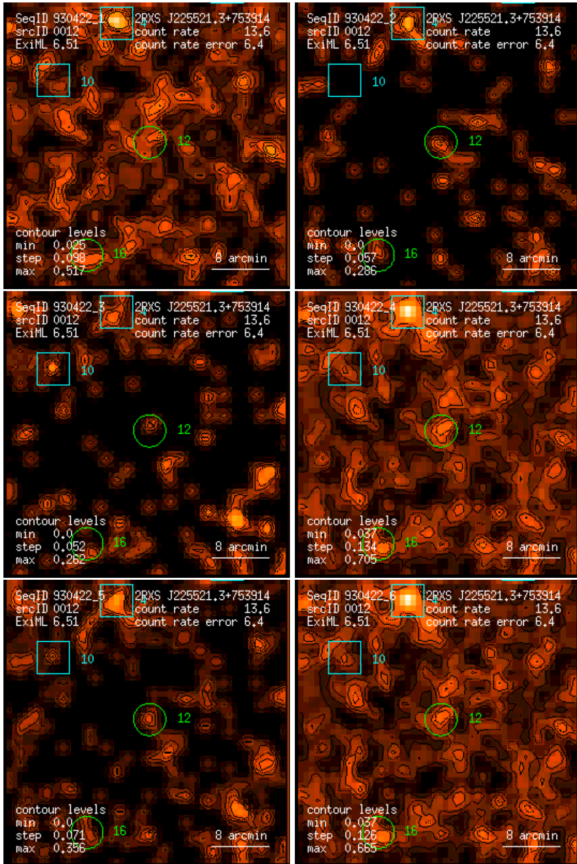
Figure 12: RASS 930422: detection 0012: band rate images, Gaussian filter: (1) PSPC channels 11 – 41, (2) 52 – 90, (3) 91 – 201, (4) 11 – 235, (5) 52 – 201, (6) 11 – 201. Broad band rates in counts/ks. Band rate contour levels in counts/ks/arcmin 2 .
