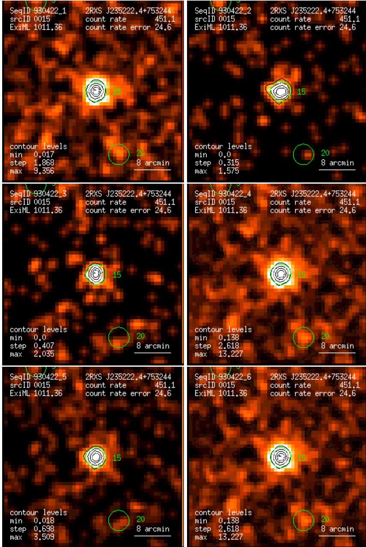
Figure 15: RASS 930422: detection 0015: band rate images, Gaussian filter: (1) PSPC channels 11 – 41, (2) 52 – 90, (3) 91 – 201, (4) 11 – 235, (5) 52 – 201, (6) 11 – 201. Broad band rates in counts/ks. Band rate contour levels in counts/ks/arcmin 2 .
