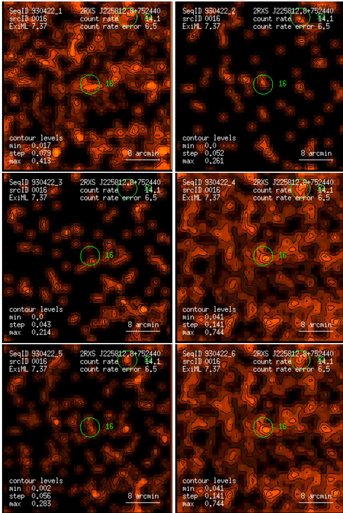
Figure 16: RASS 930422: detection 0016: band rate images, Gaussian filter: (1) PSPC channels 11 – 41, (2) 52 – 90, (3) 91 – 201, (4) 11 – 235, (5) 52 – 201, (6) 11 – 201. Broad band rates in counts/ks. Band rate contour levels in counts/ks/arcmin 2 .
