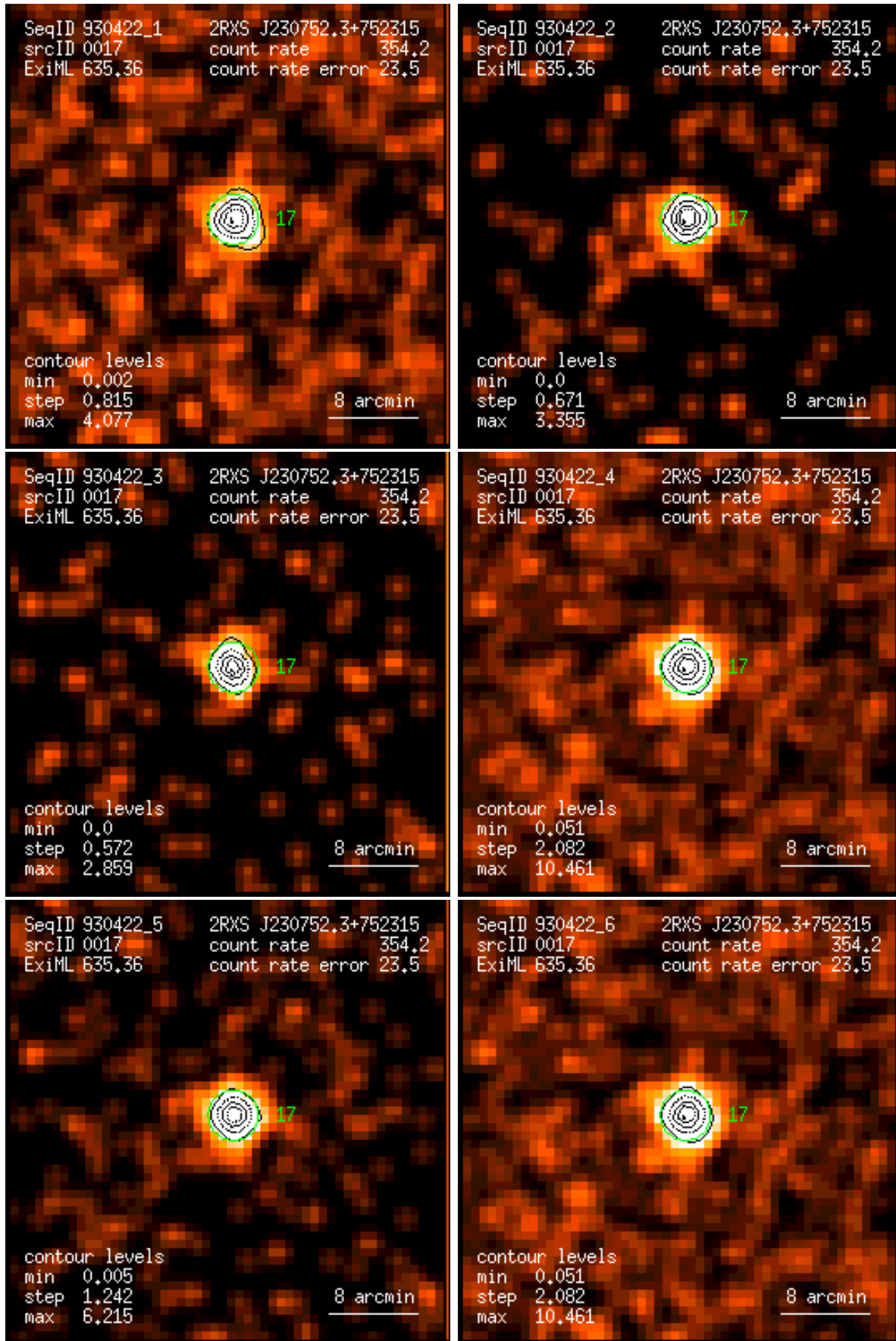
Figure 17: RASS 930422: detection 0017: band rate images, Gaussian filter: (1) PSPC channels 11 – 41, (2) 52 – 90, (3) 91 – 201, (4) 11 – 235, (5) 52 – 201, (6) 11 – 201. Broad band rates in counts/ks. Band rate contour levels in counts/ks/arcmin 2 .
