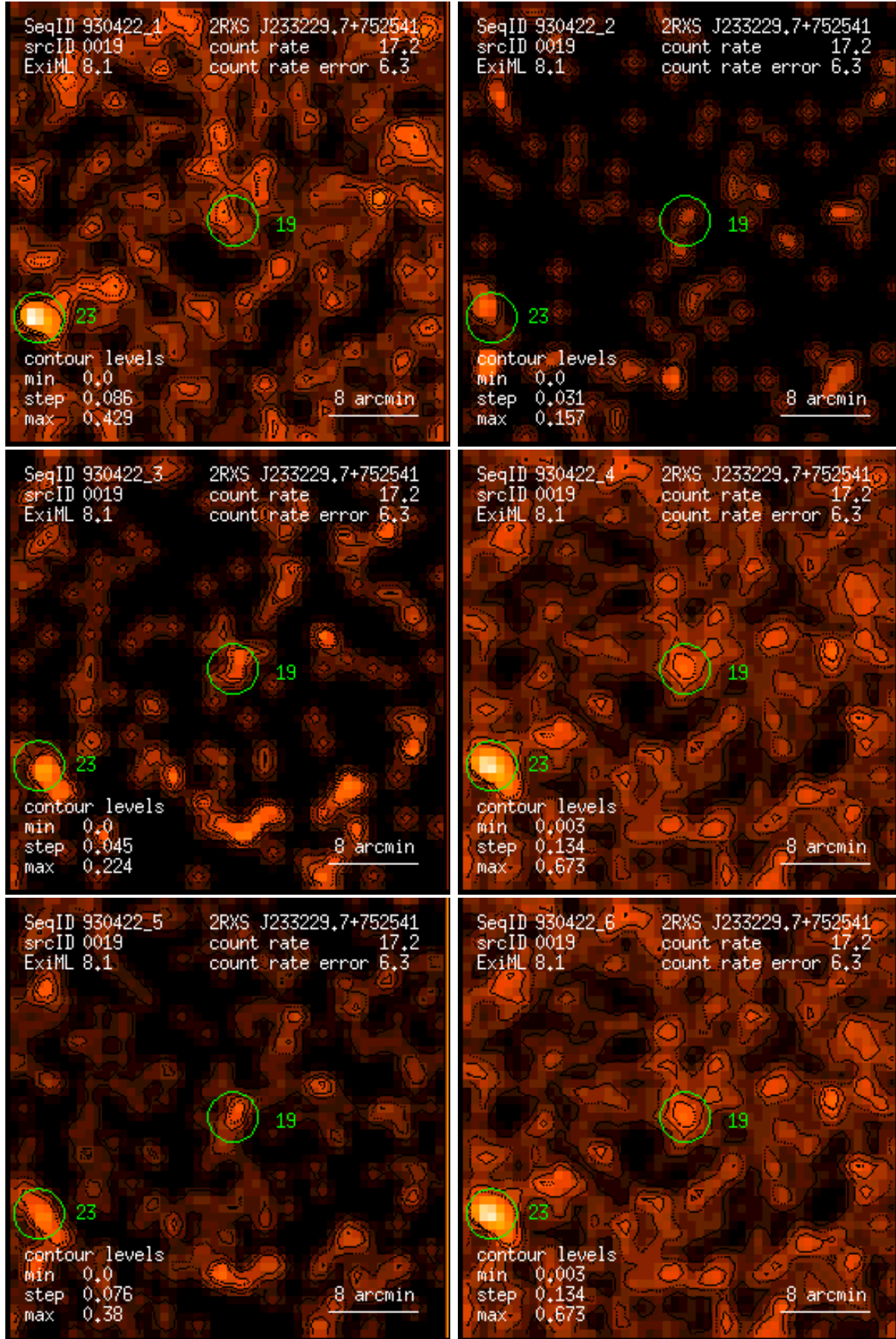
Figure 19: RASS 930422: detection 0019: band rate images, Gaussian filter: (1) PSPC channels 11 – 41, (2) 52 – 90, (3) 91 – 201, (4) 11 – 235, (5) 52 – 201, (6) 11 – 201. Broad band rates in counts/ks. Band rate contour levels in counts/ks/arcmin 2 .
