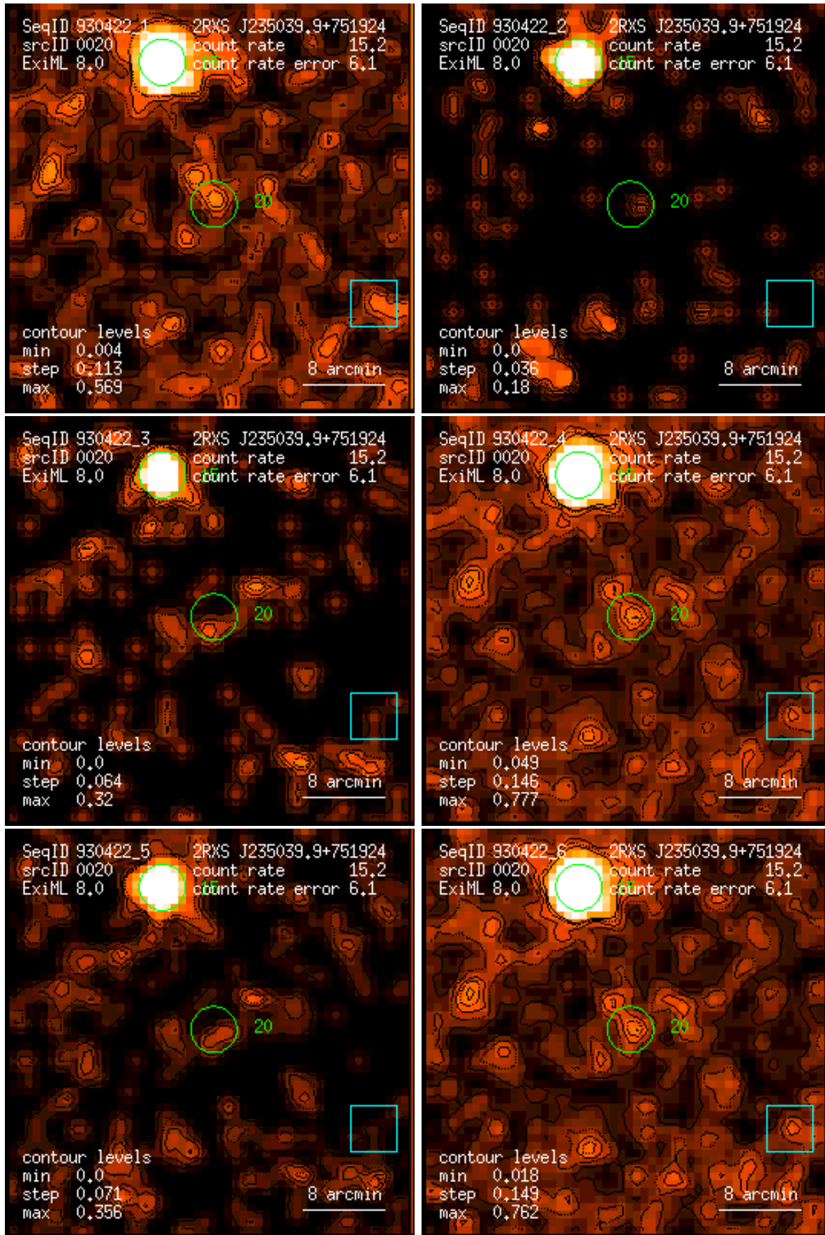
Figure 20: RASS 930422: detection 0020: band rate images, Gaussian filter: (1) PSPC channels 11 – 41, (2) 52 – 90, (3) 91 – 201, (4) 11 – 235, (5) 52 – 201, (6) 11 – 201. Broad band rates in counts/ks. Band rate contour levels in counts/ks/arcmin 2 .
