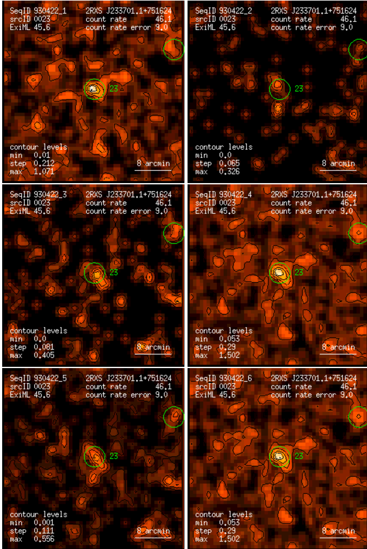
Figure 23: RASS 930422: detection 0023: band rate images, Gaussian filter: (1) PSPC channels 11 – 41, (2) 52 – 90, (3) 91 – 201, (4) 11 – 235, (5) 52 – 201, (6) 11 – 201. Broad band rates in counts/ks. Band rate contour levels in counts/ks/arcmin 2 .
