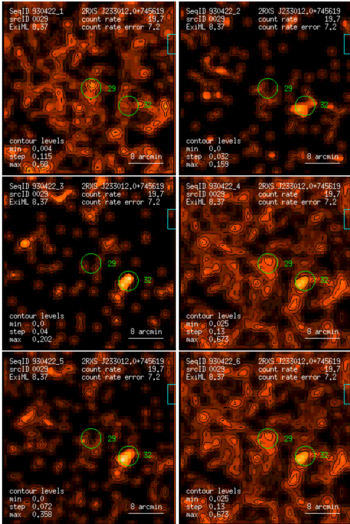
Figure 29: RASS 930422: detection 0029: band rate images, Gaussian filter: (1) PSPC channels 11 – 41, (2) 52 – 90, (3) 91 – 201, (4) 11 – 235, (5) 52 – 201, (6) 11 – 201. Broad band rates in counts/ks. Band rate contour levels in counts/ks/arcmin 2 .
