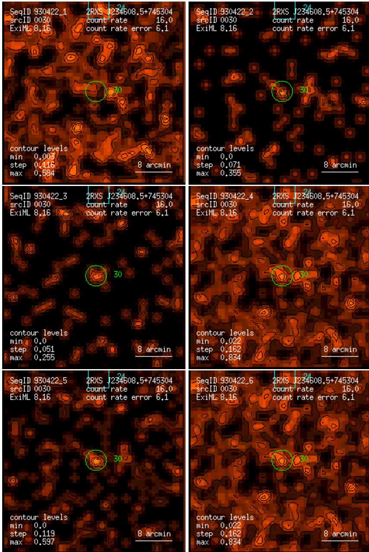
Figure 30: RASS 930422: detection 0030: band rate images, Gaussian filter: (1) PSPC channels 11 – 41, (2) 52 – 90, (3) 91 – 201, (4) 11 – 235, (5) 52 – 201, (6) 11 – 201. Broad band rates in counts/ks. Band rate contour levels in counts/ks/arcmin 2 .
