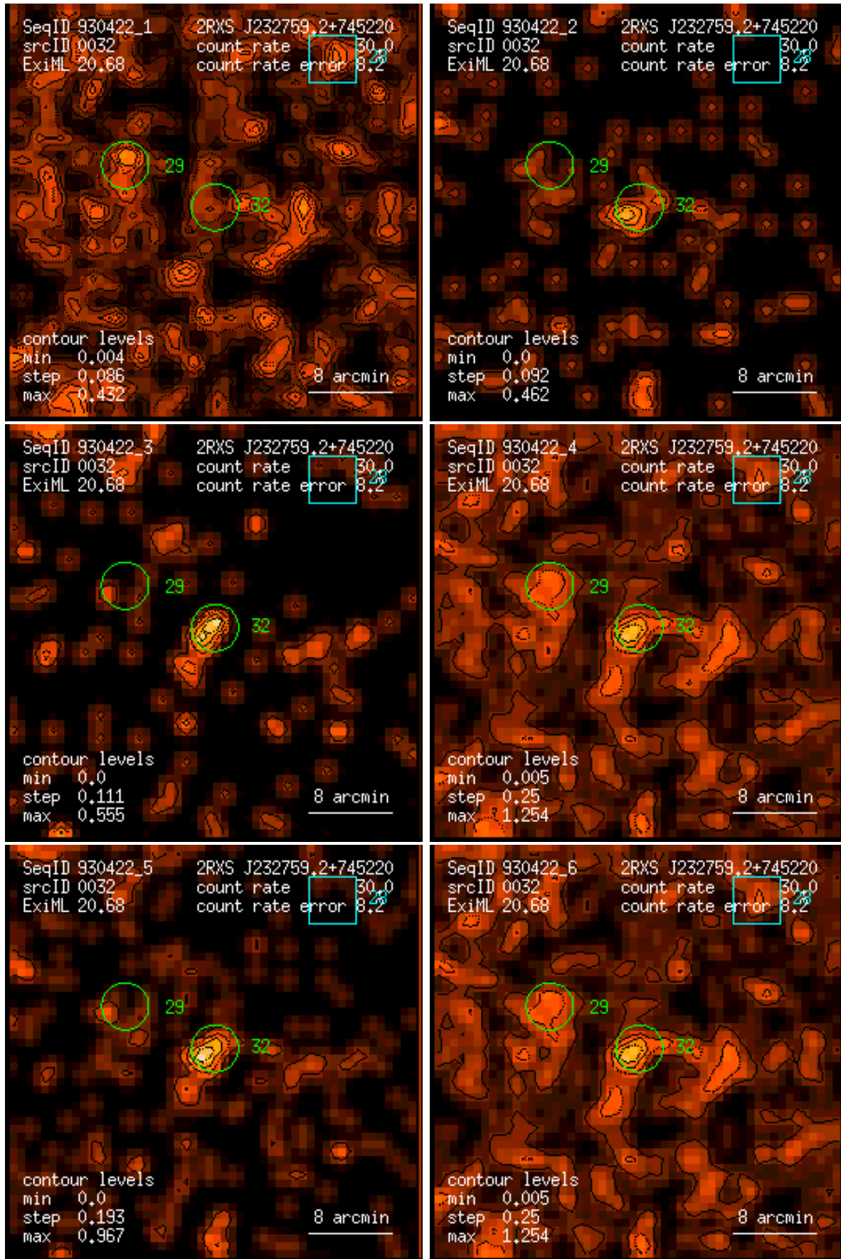
Figure 32: RASS 930422: detection 0032: band rate images, Gaussian filter: (1) PSPC channels 11 – 41, (2) 52 – 90, (3) 91 – 201, (4) 11 – 235, (5) 52 – 201, (6) 11 – 201. Broad band rates in counts/ks. Band rate contour levels in counts/ks/arcmin 2 .
