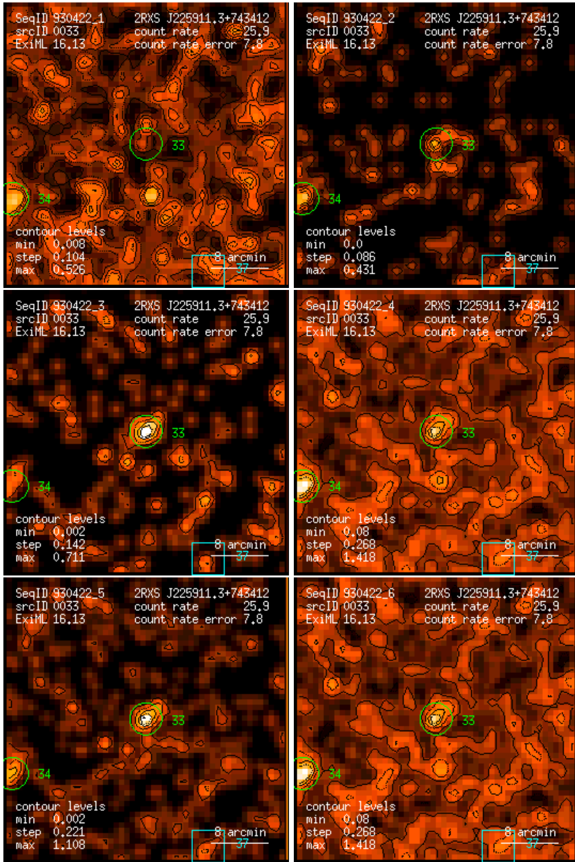
Figure 33: RASS 930422: detection 0033: band rate images, Gaussian filter: (1) PSPC channels 11 – 41, (2) 52 – 90, (3) 91 – 201, (4) 11 – 235, (5) 52 – 201, (6) 11 – 201. Broad band rates in counts/ks. Band rate contour levels in counts/ks/arcmin 2 .
